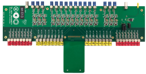
Fig. 8. The SiPM signal amplification circuit of Urs Greuter (PSI) implemented into a 16-channel card by Tel Aviv University. The top-right connector is for the amplifier 8 V input. Top blue connectors are for the SiPM voltage input and SiPM signal read-out. The bottom connectors in red are the individual SiPM HV inputs, and in yellow are the amplified signal outputs. (For interpretation of the references to colour in this figure legend, the reader is referred to the web version of this article.)
