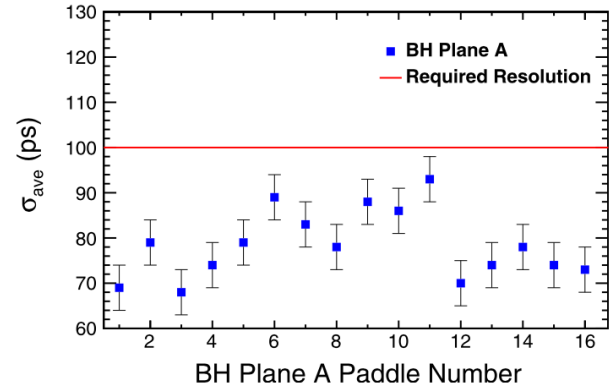
Fig. 12. Time resolution of all 16 BH-Plane-A paddles.
