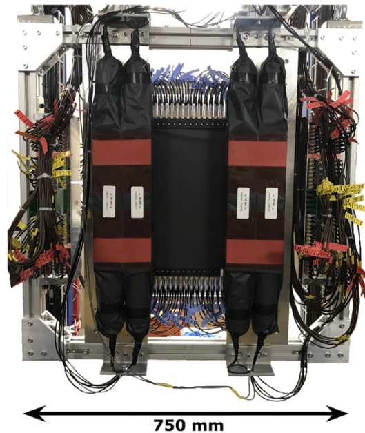
Fig. 3. Beam view of the Beam Monitor. The LEMO readout connectors of the two offset planes are seen, along with the bigger EJ-204 scintillators, and amplifiers to the sides.
