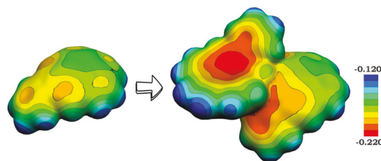
Fig. 3 Redistribuition of negative charge over \pi -surface during radical coupling, as illustrated by MEP maps of C_{26}H_{12}^{\bullet-} (left) and [\sigma-(C_{26}H_{12})_2]^{2-} (right) (PBE0/cc-pVTZ).
