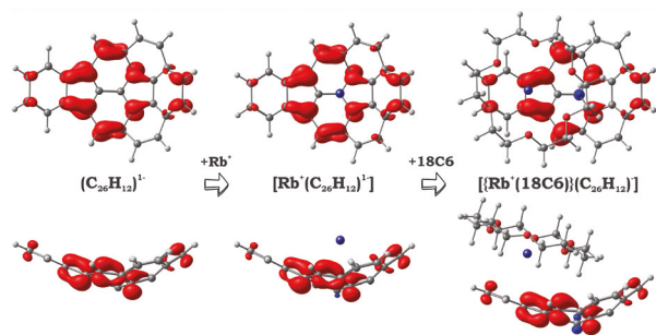
Fig. 2 Spin density distribution (isosurface 0.0035 a.u.) in indenocorannulene radical-based systems (PBE0/cc-pVTZ(C,H,O)//def2-TZVP(Rb)).
