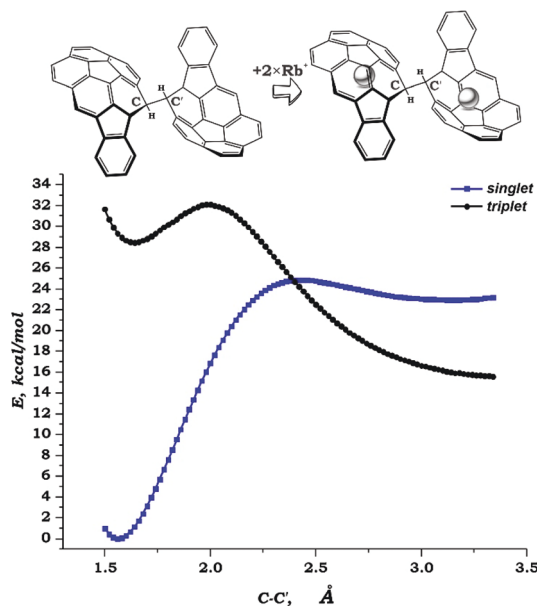
Fig. 5 Stabilization of the [\sigma-(\text{C}_{26}\text{H}_{12})_2]^{2-} dimer by \text{Rb}^+ counterions, as evidenced by PET scan for the C–C' connecting bond breaking/forming process for different spin-states (PBE0/TZVP/ZORA).
