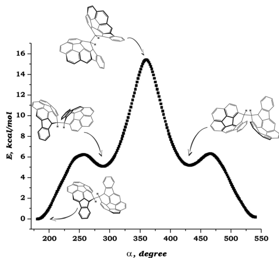
Fig. 4 Potential energy profile for the rotation of indenocorannulene fragments in [\sigma-(C_{26}H_{12})_2]^{2-} around the C-C' linker (PBE0/cc-pVTZ).
