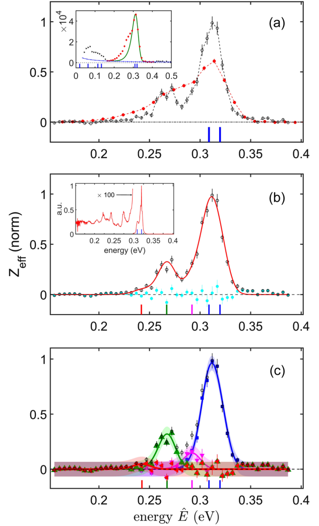
FIG. 1. The annihilation rate Z_{\text{eff}} for cyclopentane ( E_b = 48 meV) as a function of peak total energy \hat{E} . (a) Background-subtracted Z_{\text{eff}} in the region near the C-H stretch peak for the CT (open circle) and BGT (red solid circle) beams. Data in (a), (b), and (c) are normalized to the CT beam peak Z_{\text{eff}} , and dashed lines in (a) are guides to the eye. Error bars are those due to counting statistics. Inset shows absolute Z_{\text{eff}} using the BGT beam on a wider energy scale; (blue vertical bar) fundamental modes; (black right triangle) data not used in the analysis; (green curve) beam convoluted with the two fundamental C-H mode VFRs at the downshifted locations 309 and 320 meV; (blue dot-dashed line) is the background annihilation [13,24]. (b) Fits to the background-subtracted cryobeam data using three additional VFRs (beyond the C-H stretch peaks) located at 292, 267, and 242 meV (magenta, green, red vertical bars); (cyan solid circle) are the residuals. Inset shows the IR spectrum downshifted by the binding energy of 48 meV. (c) The fits to the three new resonances (magenta curve, down magenta triangle), (green curve, up green triangle), and (red curve, left red triangle), and the two C-H peaks (blue curve, blue square). For the VFR model considered here, the resonance positions are expected to be downshifted from the mode energies by E_b . Shaded regions are color coded to match the VFR and indicate the 95% confidence level.
