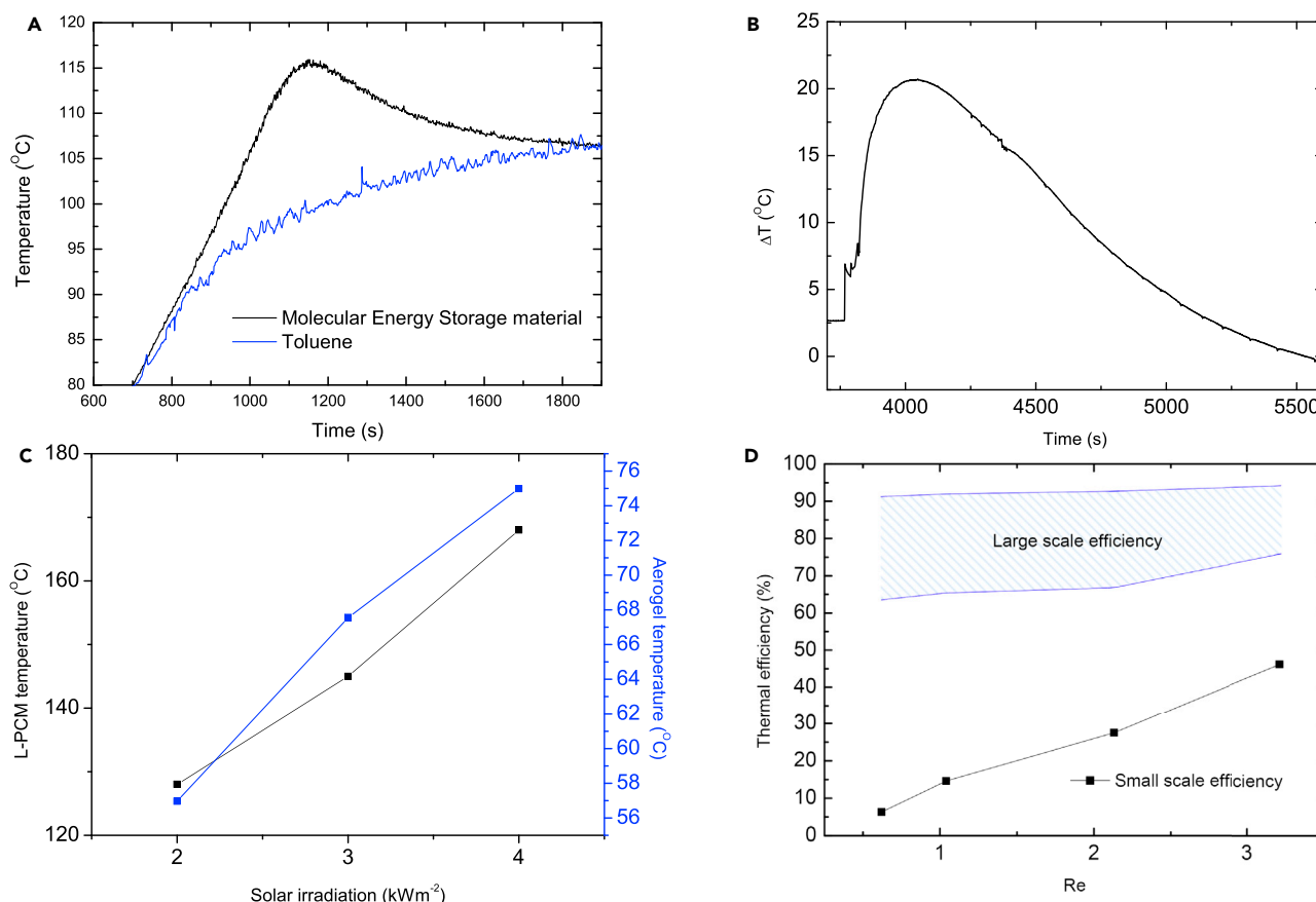
Figure 4. Full Spectrum Solar Energy Harvesting during Night
