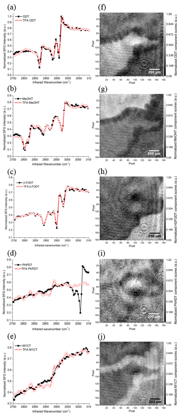
Figure 6. SFG spectra overlaid with the corresponding target transformed spectra predicted by TFA: (a) ODT, (b) MeOHT, (c) β-FODT, (d) PhPDT, and (e) M1CT. The corresponding reconstructed TFA chemical images of (f) ODT, (g) MeOHT, (h) β-FODT, (i) PhPDT, and (j) M1CT. The lighter region indicates the target SAMs. The scale bar is 200 μm.
