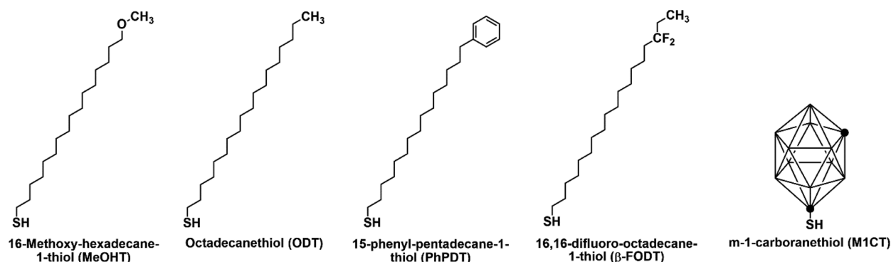
Figure 1. Respective MeOHT, ODT, PhPDT, \beta -FODT, and M1CT alkanethiol structures.
