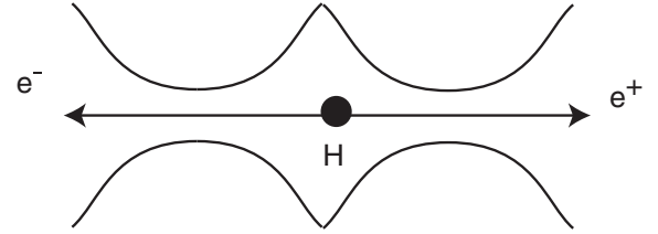
FIG. 3. A positron from one pair and an electron from the other interact in the middle and create a Higgs particle. The electron and positron at the two ends must be almost maximally entangled. However, the two initial bridges are connected into one continuous configuration with the Higgs in the middle, so the two horizons at the end do not touch. This is not consistent with the assumption 2, which implies that the horizons must touch in a maximally entangled state.
