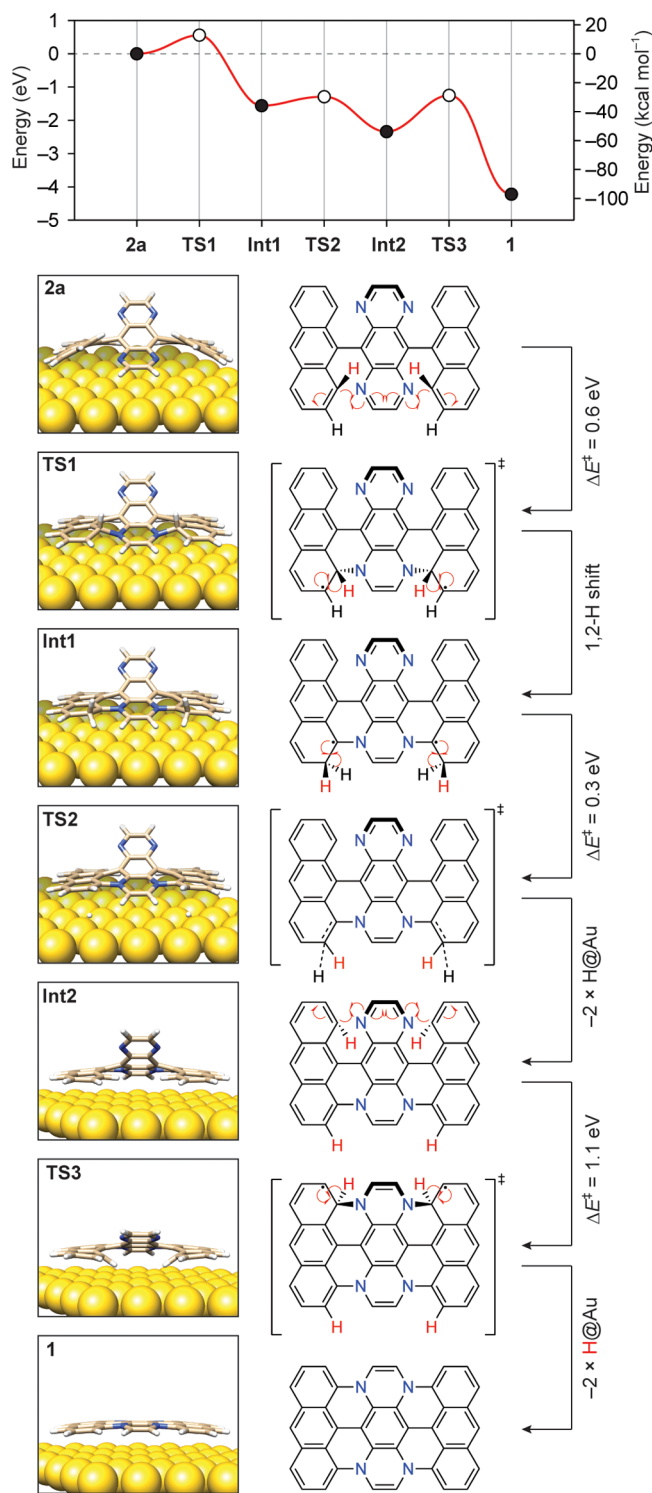
Figure 3. Calculated energy diagram for the stepwise cyclodehydrogenation of 2a to 1 . The graph shows the ab initio energy landscape for intermediates and transition states along the reaction pathway from 2a to 1 . Calculated activation energies are shown next to the reaction arrows.
