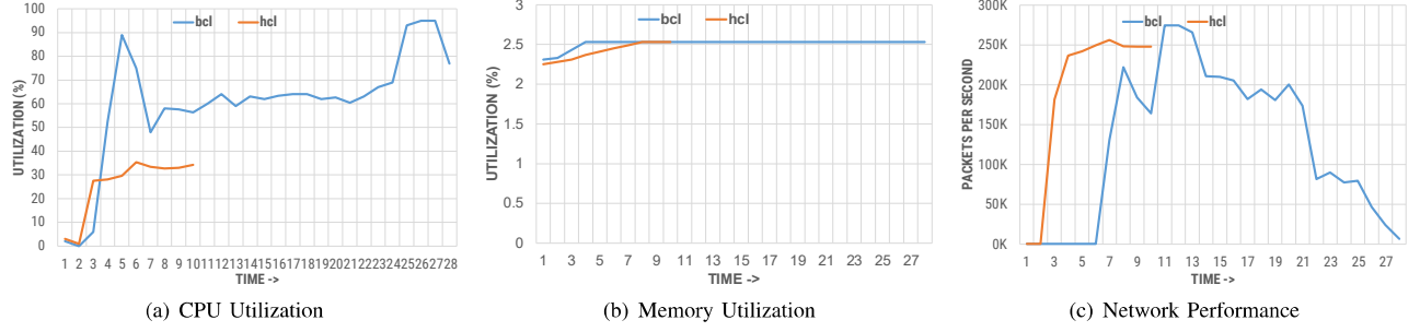
Fig. 4. Profiling of HCL and BCL
