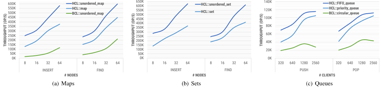
Fig. 6. Scaling HCL Data Structures.
