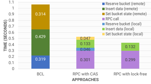
Fig. 1. Motivating test case.
