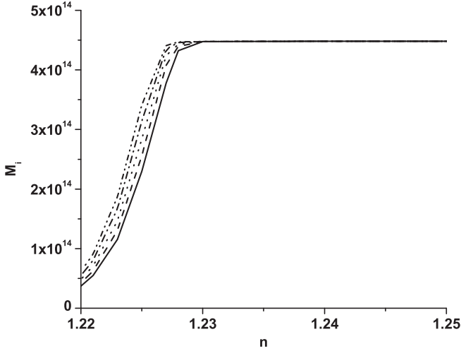
FIG. 6. This plot shows the primordial black hole masses (in grams) at the time of their formation, M_i , as a function of the spectral index, n . The solid lines represent the \mathcal{P} = 1 value for the portion of the universe which already transitioned to the new vacuum at present time. Below this line we have \mathcal{P} > 1 and the whole universe today would be destroyed. Above this line, we have \mathcal{P} < 1 , and the universe is safe. The dashed, dot, dashed dot and dashed dot dot lines represent the values \mathcal{P} = 10^{-1} , \mathcal{P} = 10^{-2} , \mathcal{P} = 10^{-3} and \mathcal{P} = 10^{-4} respectively, where the phase transition has not completed yet, but there are bubbles of true vacuum present in the universe.
