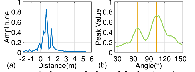
Figure 19: Performance of software defined FMCW radar.
