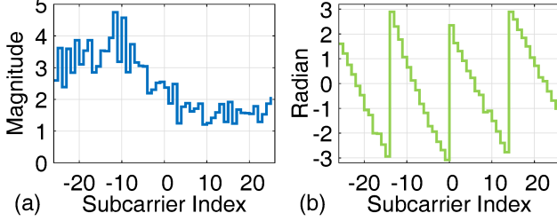
Figure 18: Example CSI measurement on one beam.
