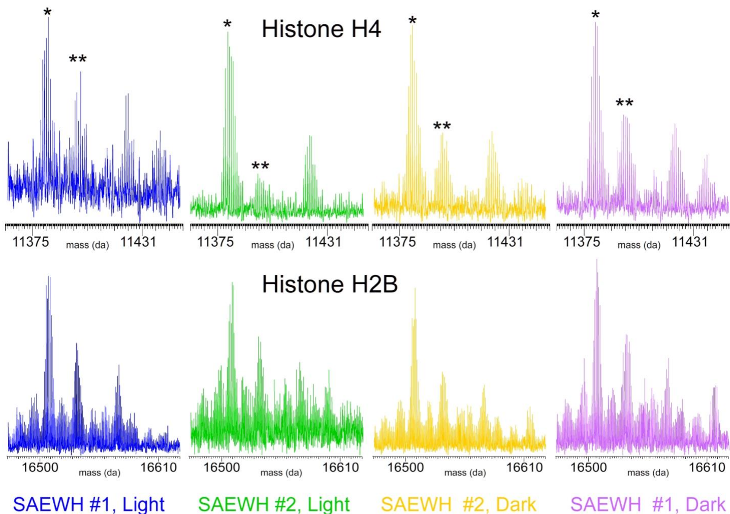
Figure 3. Exposure to light during nuclei isolation does not increase procedure-based oxidation of extracted histone H2B and H4. Harvested cell-wall-less Chlamydomonas were exposed to light (blue, green) or kept in the dark (yellow, lavender) during nuclei isolation prior to preparing salt and acid-extracted whole histones (SAEWH) and nanoLC TDMS analysis. The experiment was duplicated, from cell growth to histone extraction, and also analyzed by TDMS (blue/lavender (SAEWH #1) vs. green/yellow (SAEWH #2)). A histone H4 proteoform (N \alpha -ac, K79me1) that is unoxidized is marked with an asterisk (*), while the oxidized proteoform (N \alpha -ac, K79me1, M84ox) is marked with a double asterisk (**). These samples were also analyzed by SDS-PAGE: SAEWH #1, light (blue) = Figure 2, lane 6; SAEWH #2, light (green) = Figure 2, lane 7; SAEWH #1, dark (yellow) = Figure 2, lane 8; SAEWH #2, dark (lavender) = Figure 2, lane 9.
