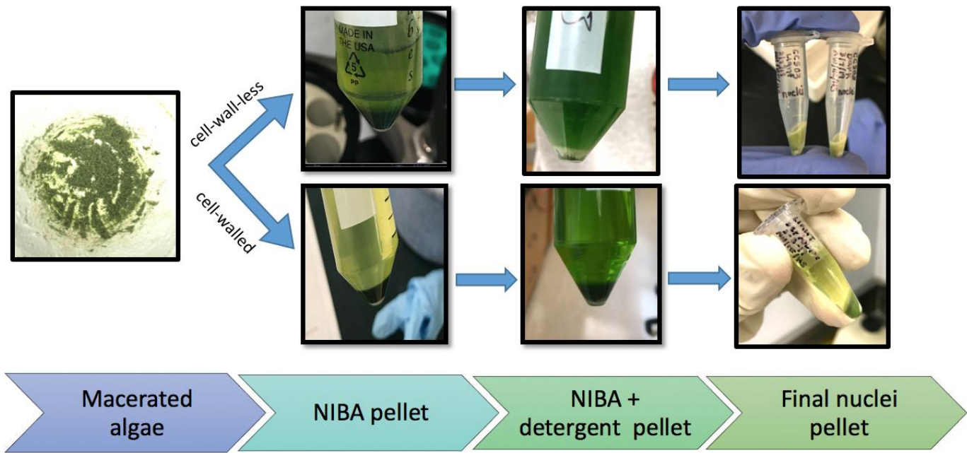
Figure 1. Representative images of the steps involved in Chlamydomonas nuclei isolation. The far left image shows finely ground algae after maceration with a mortar and pestle. Macerated cell-walled ( nzp70 D10+ ) and cell-wall-less ( cc503 ) Chlamydomonas are first washed (NIBA pellet), then lysed with detergent (NIBA + detergent pellet) and the resulting nuclei are transferred to microcentrifuge tubes prior to histone extraction (Final nuclei pellet). The final nuclei pellets show a faint green color, which is generally darker for cell-walled (bottom) than cell-wall-less Chlamydomonas (top).
