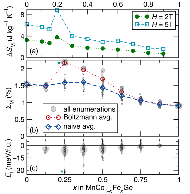
FIG. 2. Comparison of (a) peak \Delta S_M values as measured by Lin et al. for applied fields of 2 T and 5 T [37] and (b) calculated \Sigma_M vs. x for \text{Mn}(\text{Co}_{1-x}\text{Fe}_x)\text{Ge} . In (b), each gray circle represents a single enumerated cell, with the area of each circle proportional to its Boltzmann weight as calculated in equation 3. Both Boltzmann (equation 4) and naive (equation 2) averages of \Sigma_M for composition x are overlaid. (c) Energy of formation vs. x for each cell. The asterisk indicates the cell indicated as cell B in Fig. 5. The gray shaded areas (violin plot) visualize the distribution of the supercell energies.
