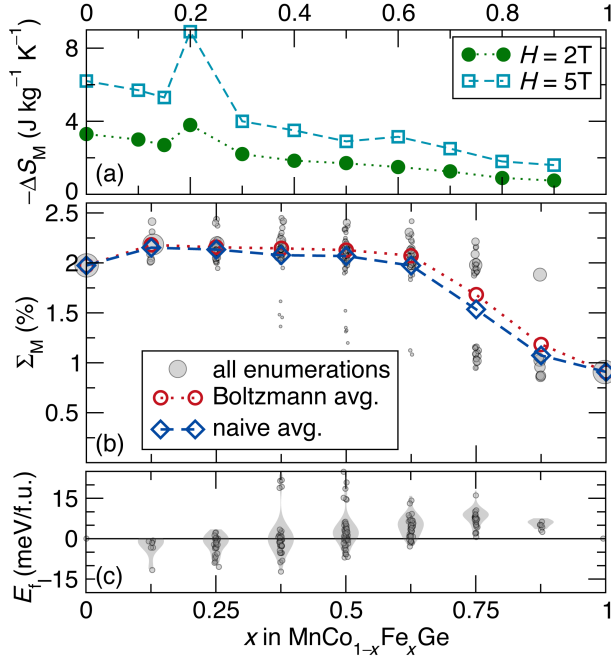
FIG. 6. Comparison of peak \Delta S_M values as measured by Lin et al. [37] (a) and calculated \Sigma_M vs. x (b) for \text{Mn}(\text{Co}_{1-x}\text{Fe}_x)\text{Ge} using global \Sigma_M values computed from calculations starting from both the orthorhombic and hexagonal structures, as discussed in the text. Please refer to the Fig. 2 caption for definitions.
