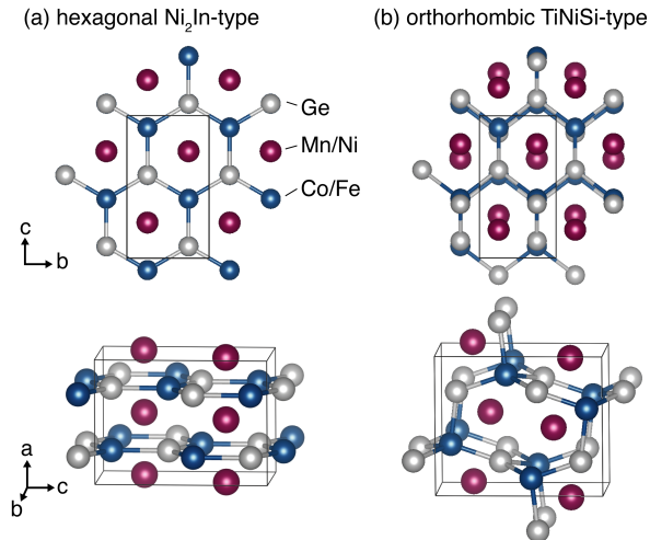
FIG. 1. Hexagonal (a) and orthorhombic (b) structure types of MnCoGe, depicted in the orthorhombic setting. The orthorhombic structure can be accessed from the hexagonal structure by a displacive phase transition involving corrugation of the honeycomb Co-Ge network.
