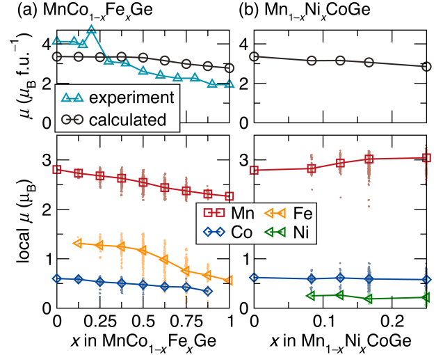
FIG. 4. Total (top) and local (bottom) evolution of the DFT magnetic moments for Mn(Co 1-x Fe x )Ge (a) and (Mn 1-x Ni x )CoGe (b). All of the individual transition metal local moments from individual enumerated cells are shown as small dots, while the Boltzmann-averaged local and total moments are shown as larger symbols connected by lines. For Mn(Co 1-x Fe x )Ge, experimentally measured 5 K saturated total magnetic moments from Lin et al. [37] are plotted for comparison.
