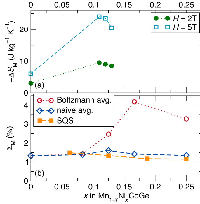
FIG. S2: (b) \Sigma_M for (\text{Mn}_{1-x}\text{Ni}_x)\text{CoGe} ( x \leq 0.25 ) calculated using special quasirandom structures (SQSs) with 48 atoms each is shown compared to \Sigma_M calculating using the supercell approach (main text Fig. 2) with either naive averaging (main text Eqn. 2) or Boltzmann averaging (main text Eqn. 4). (a) shows the experimental peak \Delta S_M for applied fields of 2 T and 5 T, as reported by Zhang et al. [3]. The SQS structure gives results similar to the naive average of the supercells.
