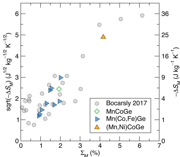
FIG. 7. Correspondence between peak values of experimental -\Delta S_M for an applied field of 5 T and magnetic deformation \Sigma_M . Gray circles show the results from Ref. 15, which considered only ordered magnets.
