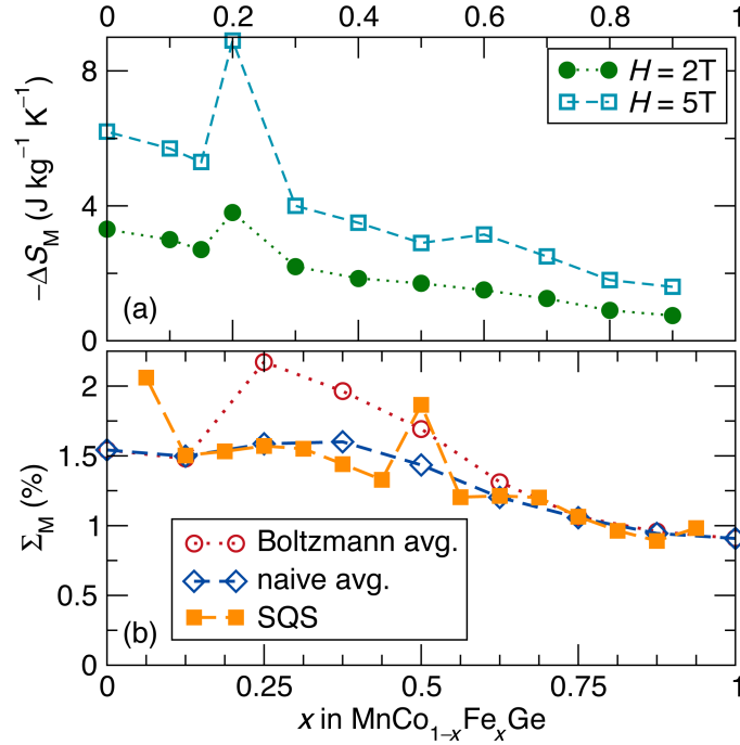
FIG. S1: (b) \Sigma_M for \text{Mn}(\text{Co}_{1-x}\text{Fe}_x)\text{Ge} calculated using special quasirandom structures (SQSs) with 48 atoms each is shown compared to \Sigma_M calculating using the supercell approach (main text Fig. 2) with either naive averaging (main text Eqn. 2) or Boltzmann averaging (main text Eqn. 4). (a) shows the experimental peak \Delta S_M for applied fields of 2 T and 5 T, as reported by Lin et al. [2]. The SQS approach gives results similar to the naive average of the supercells, with some deviations.
