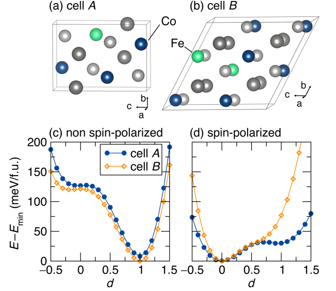
FIG. 5. Transition path energies between the hexagonal ( \text{MnFeGe} -like, d = 0 ) and orthorhombic ( \text{MnCoGe} -like, d = 1 ) structures of two different enumerated configurations of \text{MnCo}_{0.75}\text{Fe}_{0.25}\text{Ge} , (c) without and (d) with spin polarization. (a) Cell A shows a transition path landscape which is characteristic of that experienced by the majority of the enumerated cells, which remain orthorhombic after both nonmagnetic and magnetic structural relaxations. (b) Cell B is the special cell marked by an asterisk in Fig. 2, which transformed to the hexagonal structure during the spin-polarized relaxation.
