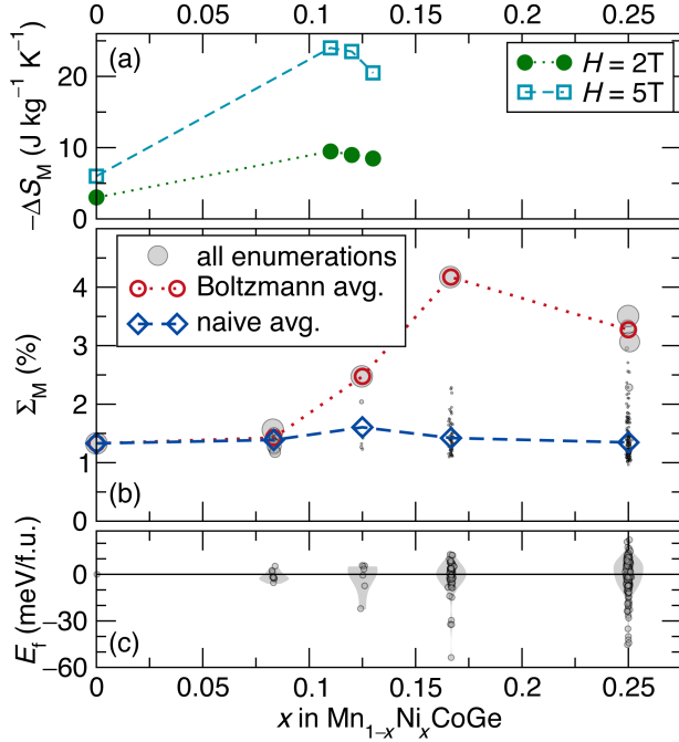
FIG. 3. Comparison of (a) experimental peak \Delta S_M values as measured by Zhang et al. [27] and (b) calculated \Sigma_M for (Mn 1-x Ni x )CoGe ( x \leq 0.25 ). (c) Energies of formation vs. x for the enumerated cells. Refer to the Fig. 2 caption for additional definitions.
