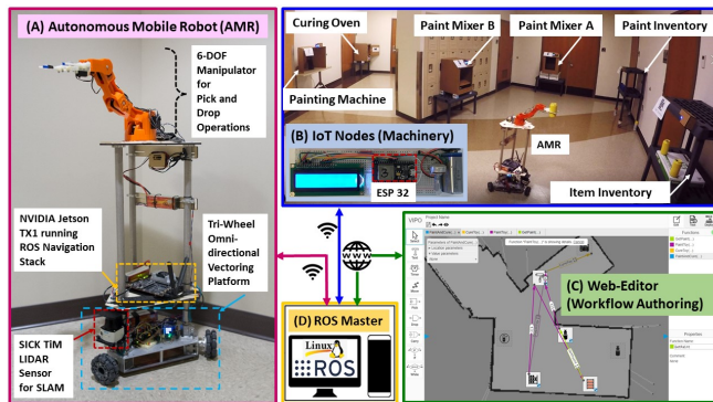
Figure 13. System Setup for the factory use-case (A) Autonomous Mobile Robot (B) IoT Nodes (industrial machinery) (C) The Vipo IDE (D) ROS Master
