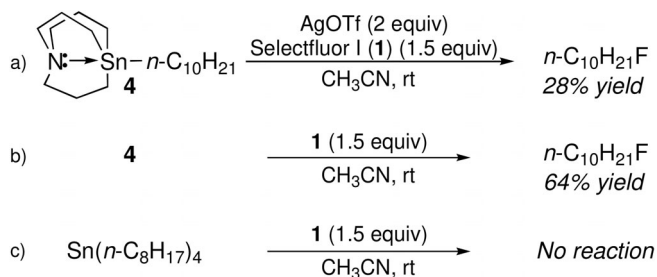
Scheme 3. Electrophilic fluorination of primary alkylstannanes with and without silver.
