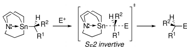
Scheme 7. Proposed mechanism of electrophilic substitution.
