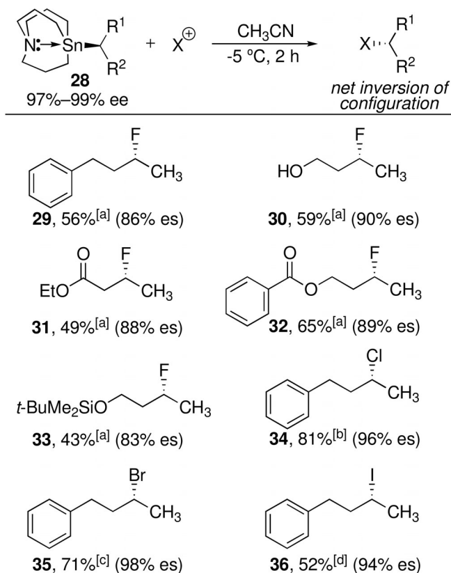
Scheme 6. Stereospecific electrophilic halogenations of enantio-enriched alkylcarbastannatranes. [a] 1 (1.5 equiv), styrene (1 equiv), pyridine (0.5 equiv); [b] TCCA (1.5 equiv); [c] NBS (1.5 equiv); [d] NIS (1.5 equiv).
