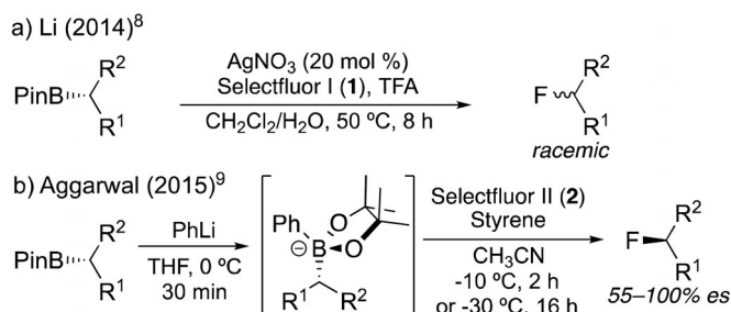
Scheme 1. Electrophilic fluorination of enantioenriched secondary alkylboron reagents.
