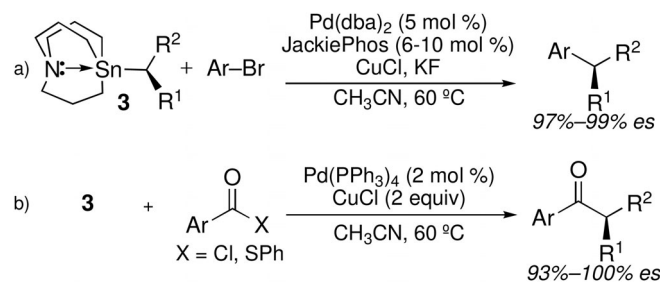
Scheme 2. Use of enantioenriched alkylcarbostannatranes in stereospecific Pd-catalyzed cross-coupling reactions.
