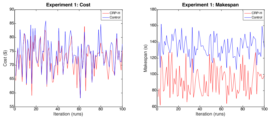
Fig. 3 Experiment 1: Operational cost (left), Makespan (right)
