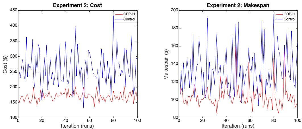
Fig. 4 Experiment 2: Operational cost (left), Makespan (right)
