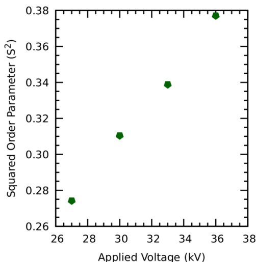
Figure 3. Calculated S^2 value of polypropylene versus the voltage used during the melt-electrospinning process employed to make the material. Data extracted from ref. [17]. For all data points, the error bars for S^2 values are within the size of the symbols.
