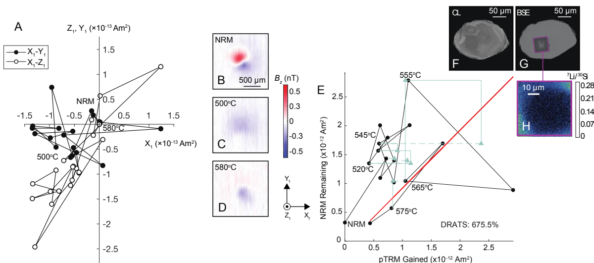
Figure 5. Paleomagnetic data for zircon grain 150107 ( 4.094 \pm 0.005 \text{ Ga} ) that passes the selection criteria but fails the paleomagnetic criteria. (A) Zijderveld diagram showing paleomagnetic direction. Closed symbols show X-Y projection of the magnetization; opened symbols show Z-Y projection of the magnetization. (B-D) Magnetic field ( B_z ) maps at a height of \sim 360 \mu\text{m} above the grains obtained with the SQUID microscope for NRM, 500°C and 580°C steps. We use a “1” subscript on X_1 , Y_1 and Z_1 to denote the fact that the grain orientation during the thermal demagnetization and paleointensity experiments is different from the grain orientation during the BSE, CL and Li measurements. (E) NRM lost versus pTRM gained during progressive laboratory heating, blue triangles show pTRM checks. Red line shows the measurements used to compute paleointensity values (550-580°C). (F-H) show CL, BSE, Li images of the grains.
