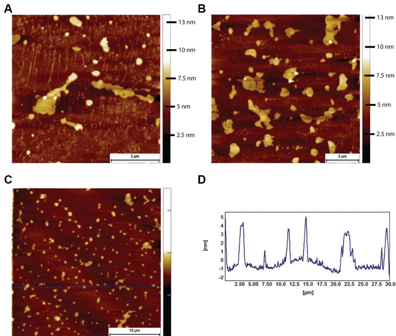
Supplementary Figure 6. AFM tapping mode images (in PBS) of naked mole-rat brain derived lipid bilayers exposed to 8 \mu\text{M} of naked mole-rat amyloid beta for 2 hr. (A and B) The bilayer is reduced to fragments of membrane, the height of fragments consistent with bilayer thickness. (C) Large scale topographic image showing the scale of the damage. (D) A height profile corresponding to the blue horizontal line in (C), confirming the height of fragments to be of bilayer thickness of 5-6 nm.
