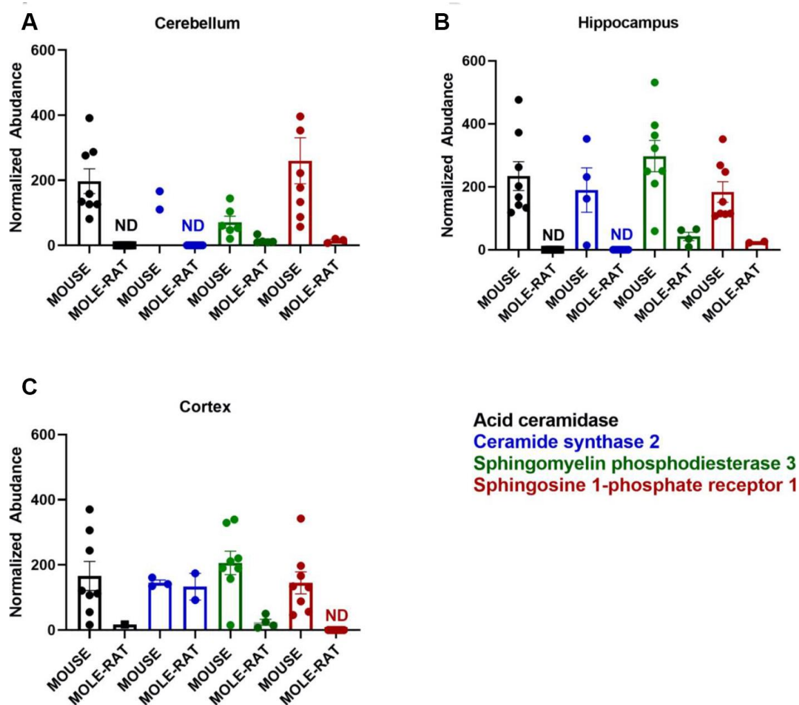
Supplementary Figure 1. Normalized abundance of proteins related to lipid metabolism and function in different brain regions in mouse and naked mole-rat. The normalized abundance of acid ceramidase, ceramide synthase 2, sphingomyelin phosphodiesterase 3 and sphingosine 1-phosphate receptor 1 are provided for cerebellum (A), hippocampus (B) and cortex (C) for mouse and naked mole-rat.
