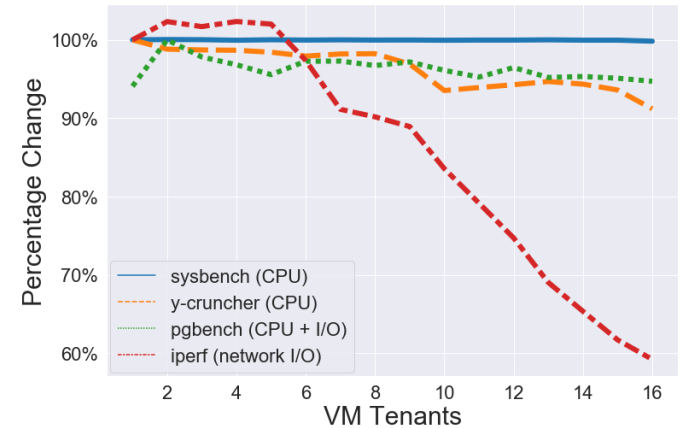
Fig. 5. 4 th generation (c4.large) Instance - Normalized Performance Degradation from VM Co-location on c4.large EC2 dedicated hosts
