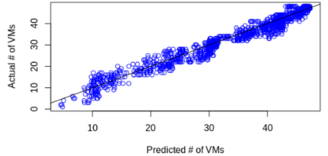
Fig. 10. Observed vs. predicted co-located VMs - random forest model
