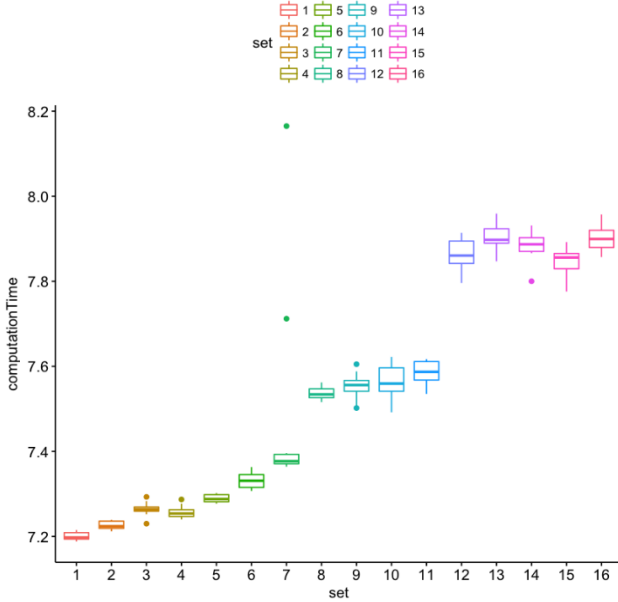
Fig. 2. This figure depicts y-cruncher average execution time when running in parallel across co-located c4.large instances using box plots. Each set includes 16 co-located VMs, where the set number refers to the number of active VMs that ran y-cruncher. All other VMs were online and idle. Box plots show the distribution of runtime for runs with a specific VM tenancy. The average runtime of y-cruncher grows with increasing tenancy by ~9.8%.
