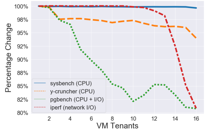
Fig. 4. 3 rd generation (c3.large) Instance - Normalized Performance Degradation from VM Co-location on c3.large EC2 dedicated hosts
