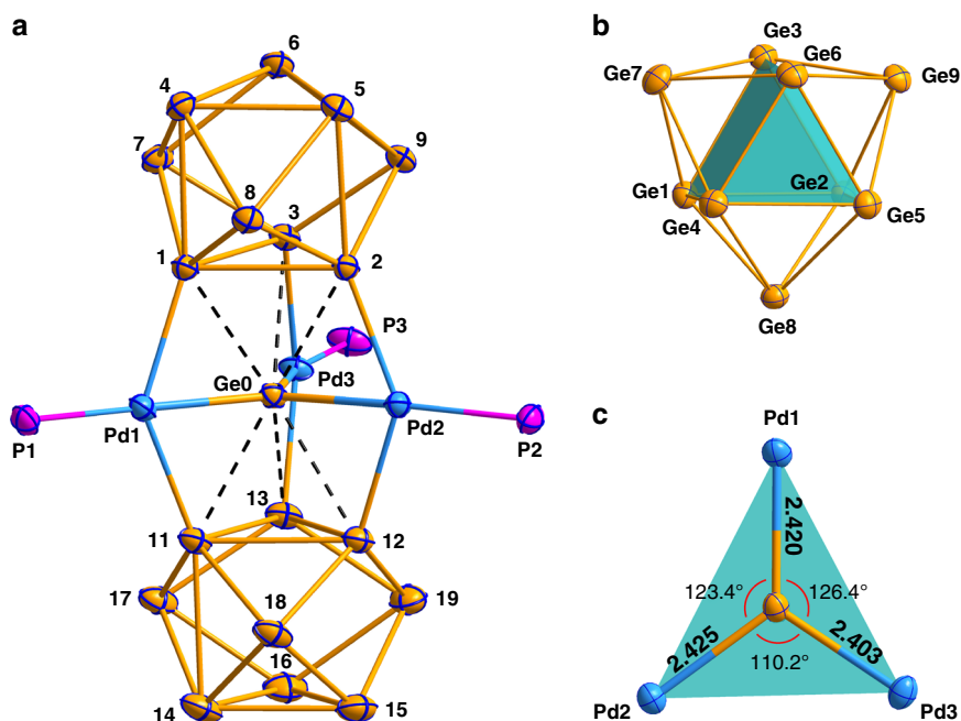
Fig. 2 Structures of the cluster-1 \{[(\text{Ge}_9)_2[\eta^6\text{-Ge}(\text{PdPPh}_3)_3]]\}^{4-} and its selected fragments. a The structure of the cluster-1, (H and C atoms are omitted for clarity, displacement ellipsoids with 35% probability). b The structure of \text{Ge}_9 subunit. c The structure of planar \text{Ge@Pd}_3 subunit. Interatomic distances are given in Å. Selected bond distances (angstroms) and angles (degrees): Ge1–Ge2: 2.744, Ge1–Ge3: 2.728, Ge2–Ge3: 2.718, Ge11–Ge12: 2.764, Ge12–Ge13: 2.751, Ge11–Ge13: 2.751, Ge4–Ge5: 2.670, Ge4–Ge6: 2.593, Ge5–Ge6: 2.619, Ge14–Ge15: 2.625, Ge14–Ge16: 2.612, Ge15–Ge16: 2.620, Ge2–Ge5: 2.808, Ge1–Ge4: 2.830, Ge3–Ge6: 3.061, Ge11–Ge14: 2.866, Ge12–Ge15: 2.893, Ge13–Ge16: 2.930 Pd1–Ge1: 2.475, Pd1–Ge11: 2.505, Pd3–Ge3: 2.533, Pd3–Ge13: 2.514, Pd2–Ge2: 2.482, Pd2–Ge12: 2.492. Ge1–Pd1–Ge11: 138.92, Ge1–Pd1–Ge0: 69.65, Ge11–Pd1–Ge0: 69.27, Ge2–Pd2–Ge12: 140.93, Ge2–Pd2–Ge0: 70.35, Ge12–Pd2–Ge0: 71.08, Ge3–Pd3–Ge13: 142.31, Ge3–Pd3–Ge0: 72.08, Ge13–Pd3–Ge0: 70.36.
