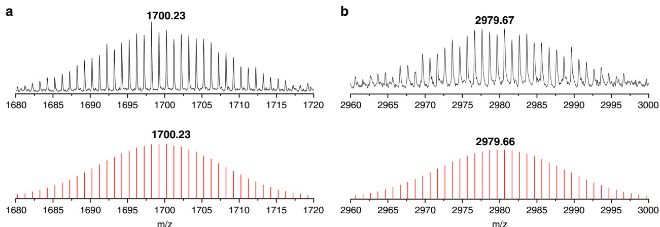
Fig. 3 Negative-ion ESI mass spectra. a Spectrum of \{(\text{Ge}_9)_2[\eta^6\text{-GePd}_3]\}^- fragment. b Spectrum of [\text{K}_3(2,2,2\text{-crypt})][\{(\text{Ge}_9)_2[\eta^6\text{-Ge(PdPPh}_3)_3]\}^-] fragment. Top: measured spectrum. Bottom: calculated spectrum.
