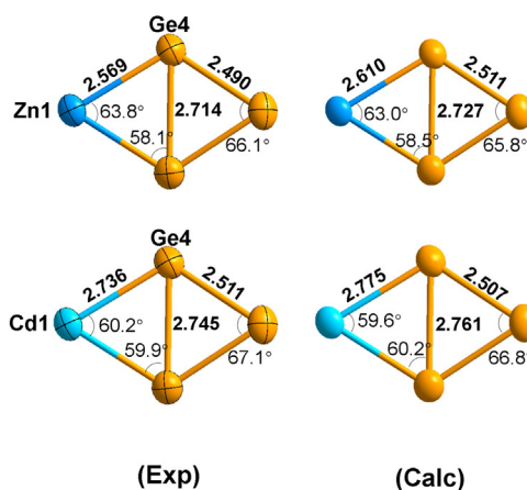
Figure 1. A) Formation scheme of [\text{M}_6\text{Ge}_{16}]^{4-} ( \text{M} = \text{Zn} or \text{Cd} ); B) Ellipsoid plot (50% level) of the crystal structure of [\text{Zn}_6\text{Ge}_{16}]^{4-} (the same structure for [\text{Cd}_6\text{Ge}_{16}]^{4-} ); C) The experimental and computed geometries of the \text{Ge}-\text{Ge}_2-\text{M} unit in [\text{M}_6\text{Ge}_{16}]^{4-} and the average distances of \text{Ge}-\text{M} and \text{Ge}-\text{Ge} are given in Å.
