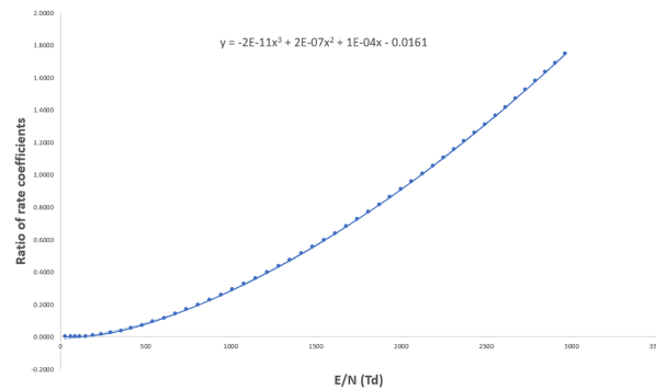
FIG. B6: Ratio of coefficients of electron impact excitations versus E/N (Td)
