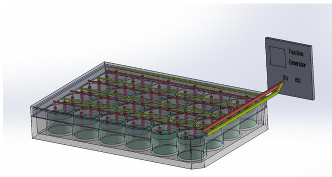
FIG. 1: Schematic of TTFields device setup based on a 24-well cell culture plate
