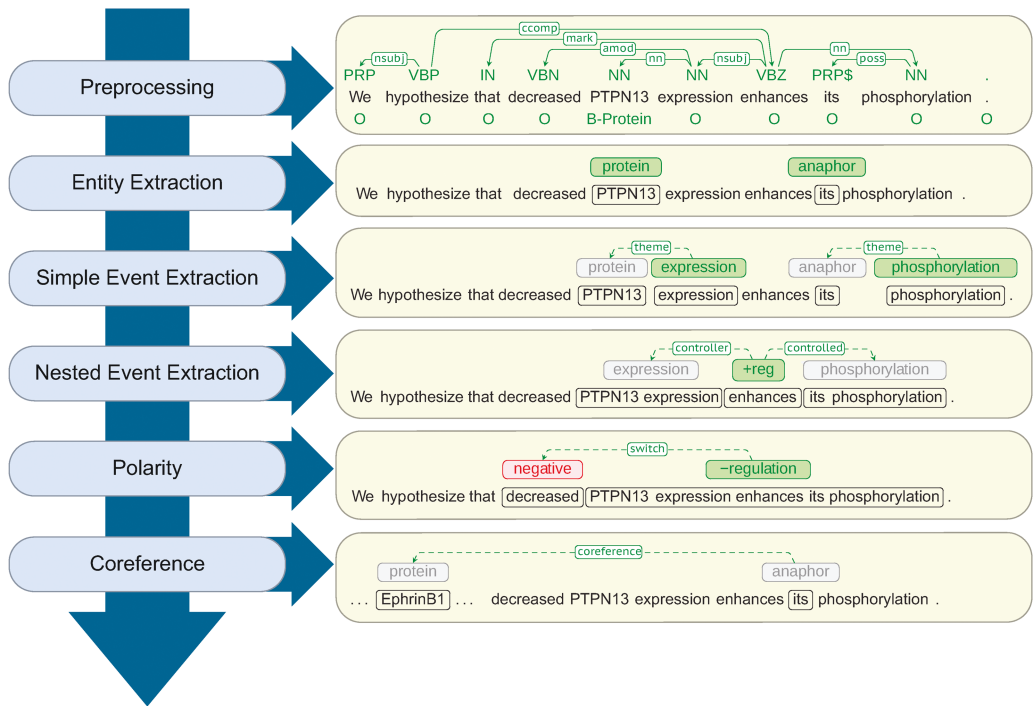
Figure 2. Architecture of the Reach system together with a walk-through example.
