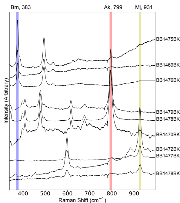
Figure 1. Raman spectra of the samples recovered from the Large-Volume Press (LVP) runs: The vertical lines highlight the key peaks for the identification of Bm (blue) at 383 \text{cm}^{-1} , Ak (red) at 799 \text{cm}^{-1} , and Mj (yellow) at 931 \text{cm}^{-1} . An LVP run ID is provided to each spectrum (Table 1).
