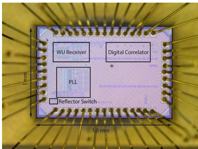
Figure 20.1.7: Micrograph of the backscatter chip.
