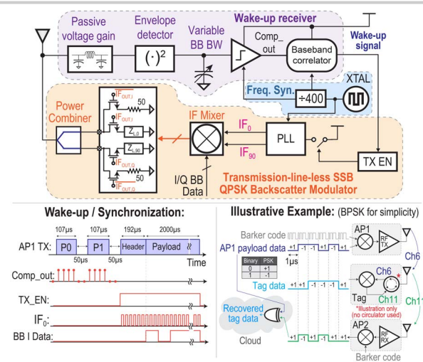
Figure 20.1.2: Block diagram of the proposed backscatter-based IoT tag (top); wake-up/synchronization and backscatter timing (bottom left); BPSK-based example of how tag data is decoded in the cloud (bottom right).
