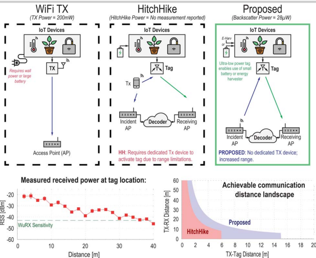
Figure 20.1.1: Proposed WiFi-compliant backscatter approach in contrast to existing art (top); measured RX power at tag location, indicating >30m wake-up range (bottom left); and achievable communication distance landscape.
