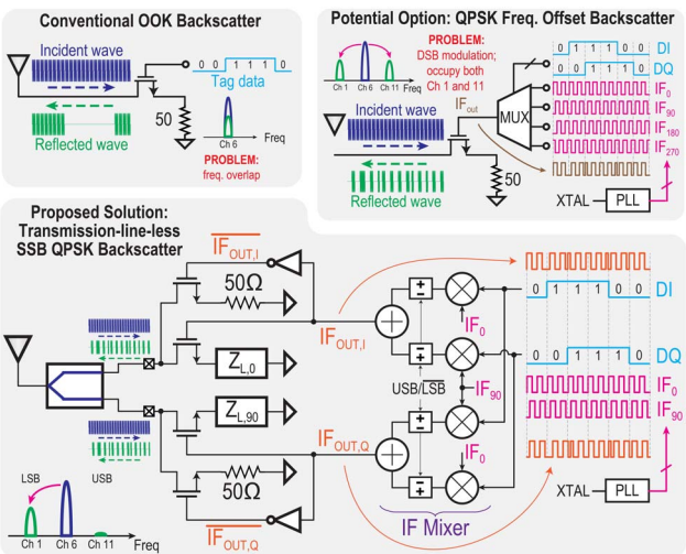
Figure 20.1.3: Methods to perform on-chip backscatter modulation: conventional frequency-overlapped OOK (top left); frequency-offset QPSK (top right); and the proposed transmission-line-less SSB QPSK approach (bottom).
