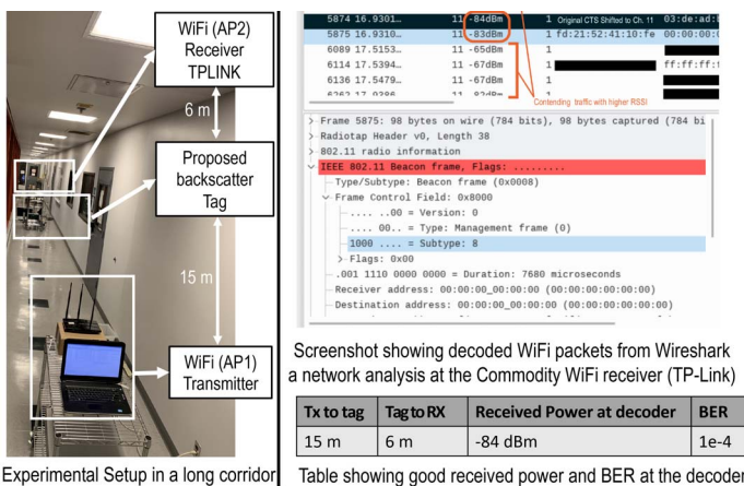
Figure 20.1.5: Wireless experimental setup (left); network analysis tool showing decoded backscatter packet with commodity WiFi RX (right).
