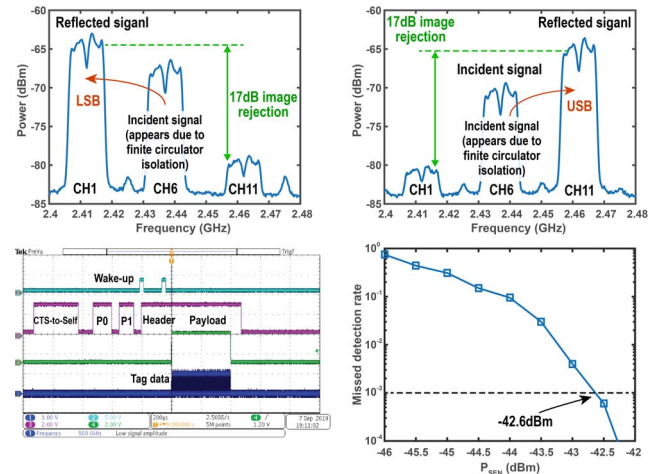
Figure 20.1.4: Measured spectrum showing SSB backscatter-based frequency translation to lower (top left) and upper (top right) sidebands with 17dB image rejection; measured wake-up and backscatter sequence (bottom left); measured missed detection rate for the WuRX (bottom right).
