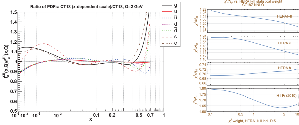
Figure 1: Left: The ratios of the candidate CT18 NNLO PDFs obtained with the x -dependent and standard factorization scales in DIS data sets. Right: The \chi^2/N_{pt} values for four HERA data sets in the CT18Z fits with the x -dependent DIS factorization scale and varied statistical weight of the HERA I +II inclusive DIS data set.
