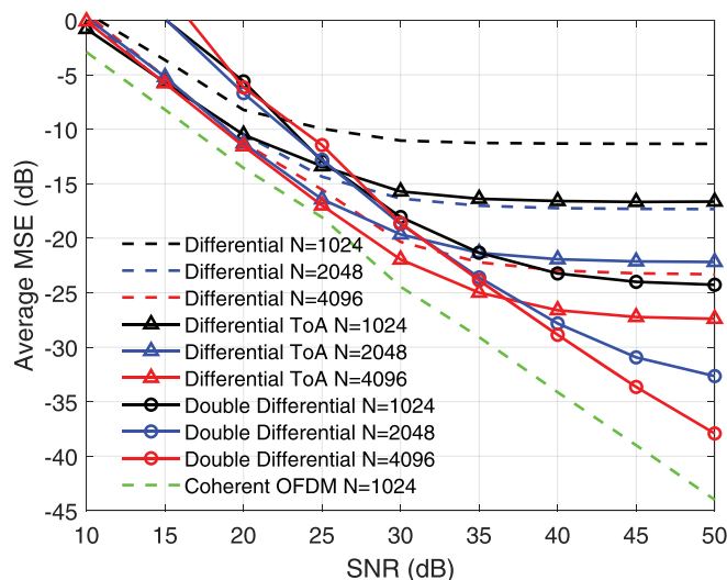
Fig. 3. (Color online) Average MSE performance versus received SNR.
