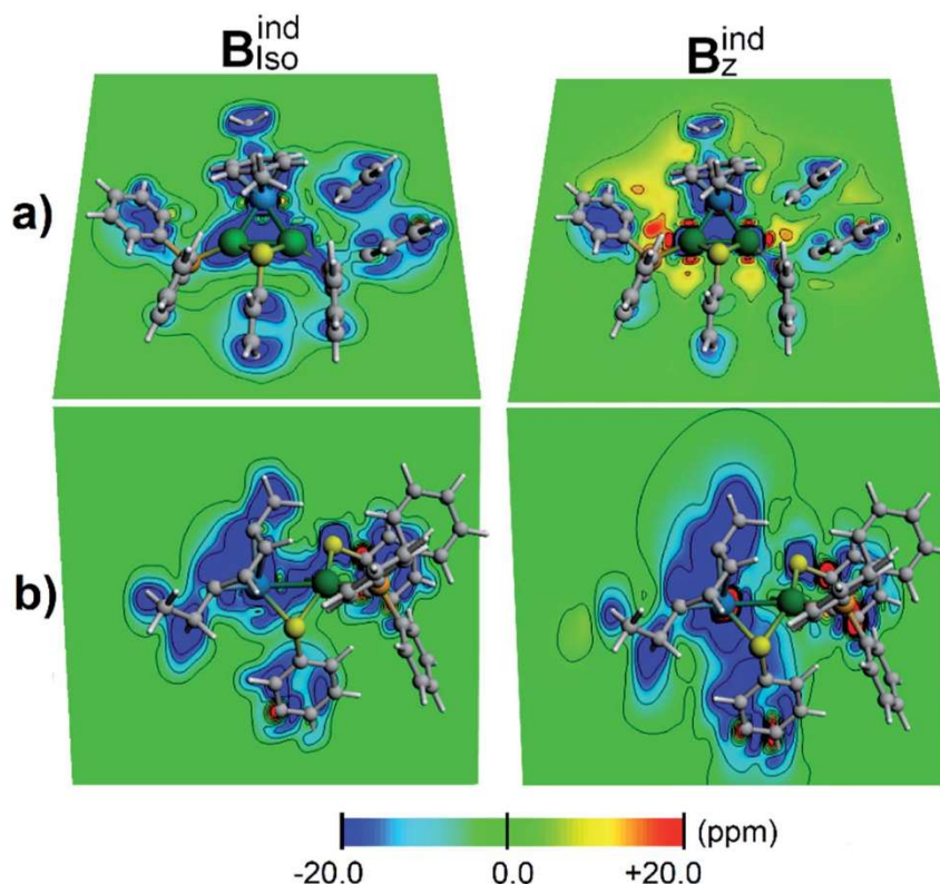
Fig. 7 Induced magnetic field of 1a denoting B_{\text{iso}}^{\text{ind}} and B_z^{\text{ind}} oriented perpendicularly to the [Pd 2 Ru] + plane. Two views are given: (a) contour plot contained in the [Pd 2 Ru] + plane and (b) bisecting the Pd–Pd bond. Blue, shielding; red, deshielding. Ru is blue and Pd is green.
