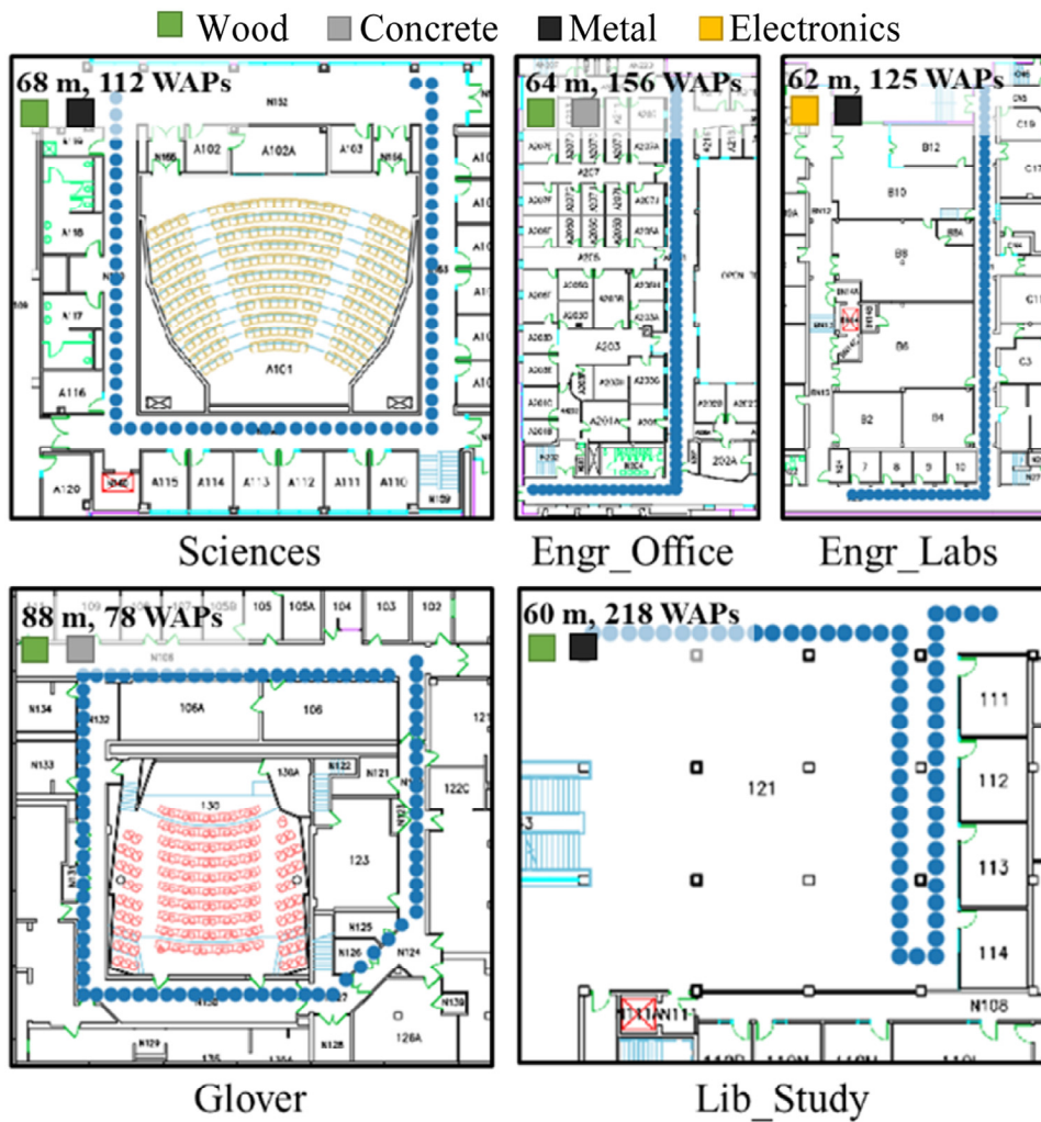
Fig. 1. Benchmark paths for indoor localization (with path lengths and WAP density, and salient path features).
