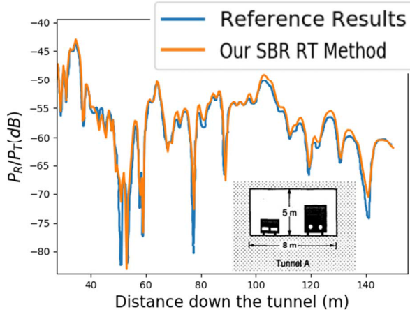
Fig. 1. Received/transmitted power along a rectangular tunnel ( \epsilon_r = 5.5 , \sigma = 0.03\text{ S/m} ) excited with a vertically polarized half-wave dipole transmitter at 1\text{ GHz} : comparison of our SBR RT method and an SBR algorithm with IT path corrections from [7].
