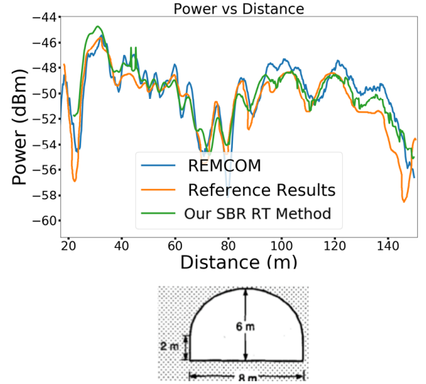
Fig. 2. Power [dBm] down the length of an arched tunnel (the tunnel cross section is shown; \sigma = 0.03\text{ S/m} , \epsilon_r = 5.5 ; excitation: vertically polarized dipole antenna at 1\text{ GHz} ): comparison of our SBR RT method with the results by the hybrid SBR/IT RT solution [7] and by the commercial REMCOM Wireless InSite solver.
