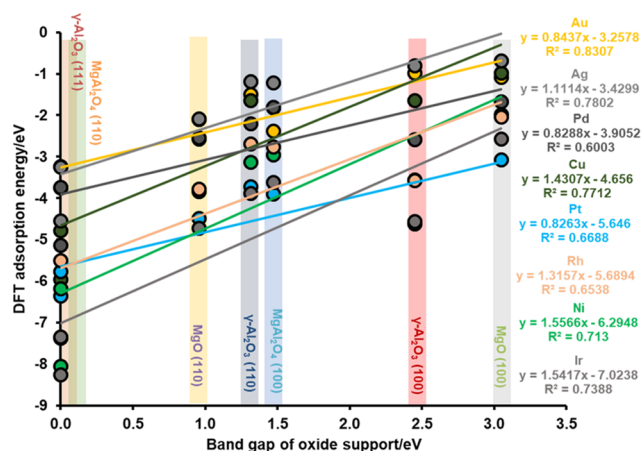
Figure 8. Relationship between DFT metal adsorption energy and band gap of the oxide support.
