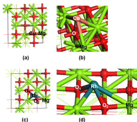
Figure 4. Cu adsorption on MgO(100) from (a) top view, (b) side view; Rh adsorption on MgO(100) from the respective (c) top view, (d) side view. Copper atoms represent Cu, blue atoms Rh, green atoms Mg, and red atoms O.
