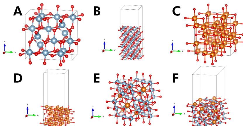
Figure 1. Structures of (a) \gamma - \text{Al}_2\text{O}_3 bulk, (b) \gamma - \text{Al}_2\text{O}_3(100) facet, (c) MgO bulk, (d) MgO(100) facet, (e) \text{MgAl}_2\text{O}_4 bulk, and (f) \text{MgAl}_2\text{O}_4(100) facet. Orange atoms represent Mg, gray atoms represent Al, and red atoms represent O.
