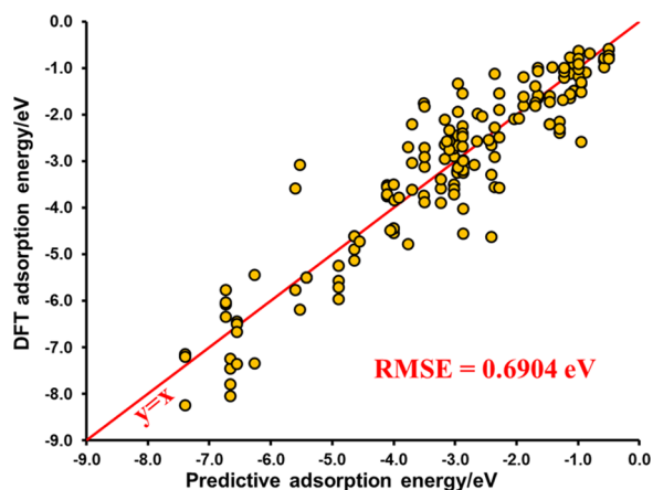
Figure 9. DFT adsorption energy versus predictive adsorption energy calculated by eq 3.
