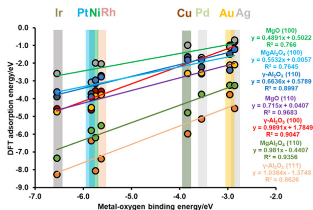
Figure 7. Relationships between DFT-calculated metal adsorption energy on each surface facet and metal–oxygen binding energy of the supported SAC.
