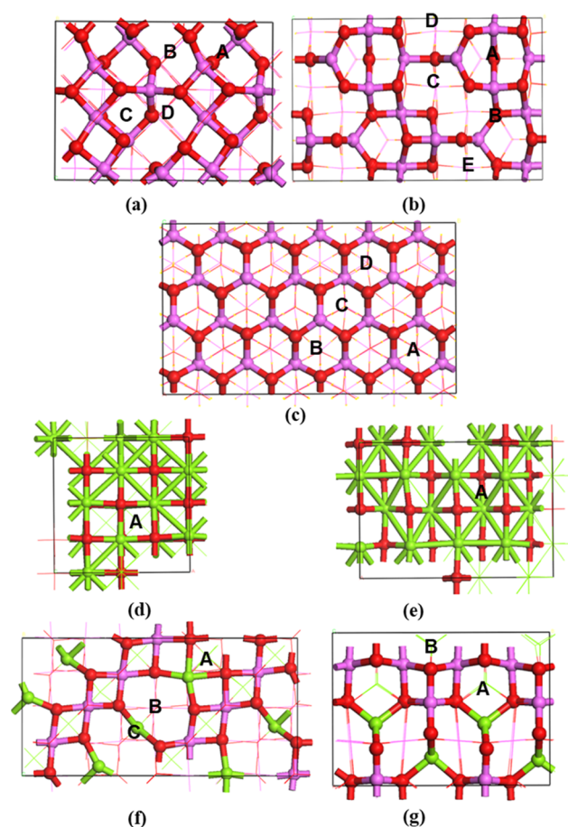
Figure 2. Chosen sites on the lowest energy termination of (a) \gamma - \text{Al}_2\text{O}_3(100) , (b) \gamma - \text{Al}_2\text{O}_3(110) , (c) \gamma - \text{Al}_2\text{O}_3(111) , (d) MgO(100), (e) MgO(110), (f) \text{MgAl}_2\text{O}_4(100) , and (g) \text{MgAl}_2\text{O}_4(110) . Sites are indicated with capital letters. Only top layers are shown by ball-and-stick, the atoms in the subsurface are shown by a wireframe. Green atoms represent Mg, pink atoms Al, and red atoms O.
