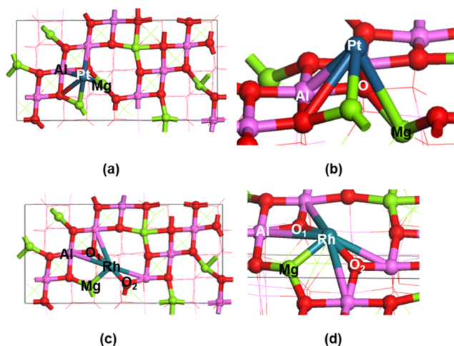
Figure 5. Pt adsorption on \text{MgAl}_2\text{O}_4(100) (a) top view, (b) side view; Rh adsorption on \text{MgAl}_2\text{O}_4(100) (c) top view, (d) side view. Dark blue atoms represent Pt, light blue Rh, green Mg, pink Al, and red O.
