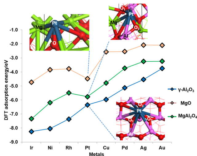
Figure 6. DFT-calculated metal adsorption energy for most preferred sites of different transition metals adsorbed on different supports; the structures of Pt adsorption are attached for an insight into the structures. Blue atoms represent Pt, green atoms represent Mg, pink atoms represent Al, and red atoms represent O.
