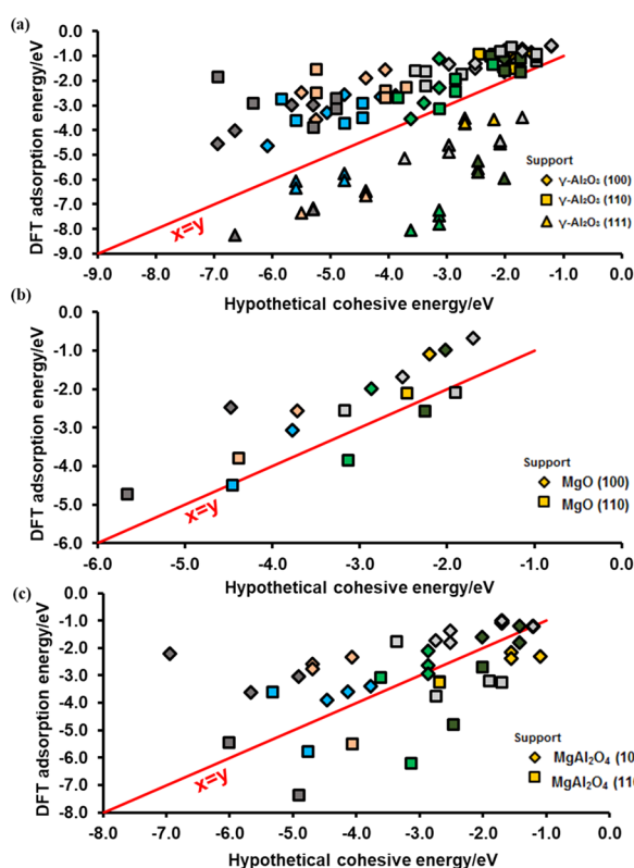
Figure 10. DFT adsorption energy vs hypothetical cohesive energy of the supported metal on (a) \gamma\text{-Al}_2\text{O}_3 , (b) \text{MgO} , and (c) \text{MgAl}_2\text{O}_4 .
