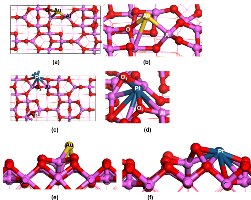
Figure 3. Au adsorption on \gamma\text{-Al}_2\text{O}_3(110) (a) top view, (b) side view; Pt adsorption on \gamma\text{-Al}_2\text{O}_3(110) (c) top view, (d) side view. Surface restructuring is observed by comparing side views of the \gamma\text{-Al}_2\text{O}_3(110) support surface when interacting with (e) Au and (f) Pt. Yellow atoms represent Au, blue atoms Pt, pink atoms Al, and red atoms O.
