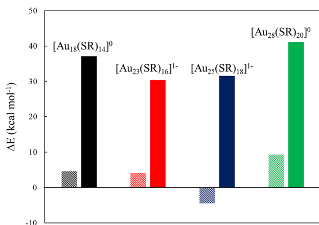
Fig. 2 Change in electronic reaction energy ( \Delta E ) for a single ligand -\text{R} (striped bars) or -\text{SR} removal (solid bars) from [\text{Au}_n(\text{SR})_m]^q nanoclusters (with \text{R}=\text{CH}_3 ). \Delta E values (in \text{kcal mol}^{-1} ) are calculated based on hydrogenation reactions of Eqs. 1 and 2
