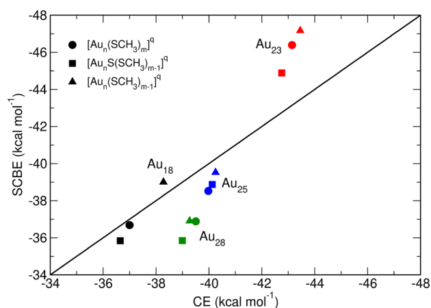
Fig. 3 Parity plot between the shell-to-core binding energy (SCBE) and core cohesive energy (CE) upon -\text{R} or -\text{SR} removal. Circles, squares, and triangles indicate the SCBE-CE of the original [\text{Au}_n(\text{SR})_m]^q , the [\text{Au}_n\text{S}(\text{SR})_{m-1}]^q and the [\text{Au}_n(\text{SR})_{m-1}]^q NCs respectively. Black, red, blue, and green colors are used to identify the fully and partially protected \text{Au}_{18} , \text{Au}_{23} , \text{Au}_{25} , and \text{Au}_{28} NCs, respectively
