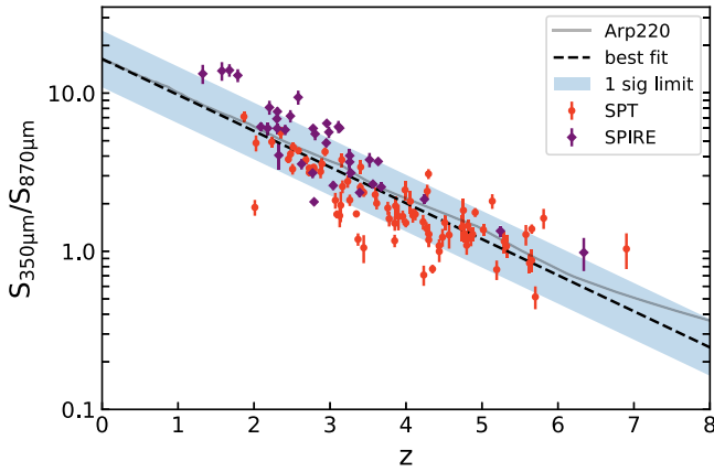
Figure 7. The S_{350\mu\text{m}}/S_{870\mu\text{m}} color serves as a rough indicator for redshift. The SPT catalog is compared to Herschel/SPIRE sources and is well described by an exponential fit with a term to describe the intrinsic scatter. The Arp220 colors were obtained by artificially observing the Arp220 SED (Silva et al. 1998) for a range of redshifts.
