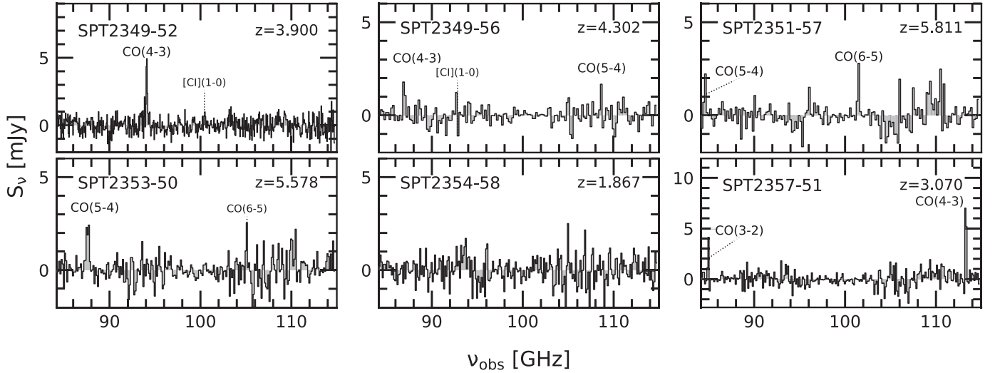
Figure B5. The 3 mm ALMA spectra (spanning 84.2–114.9 GHz) of all SPT DSFGs. Marginal detections ( >3\sigma ) are designated by the smaller font and dashed line. No spectroscopic lines were detected in SPT2354-58 because it falls into a spectroscopic redshift desert, depicted in Figure 2.
