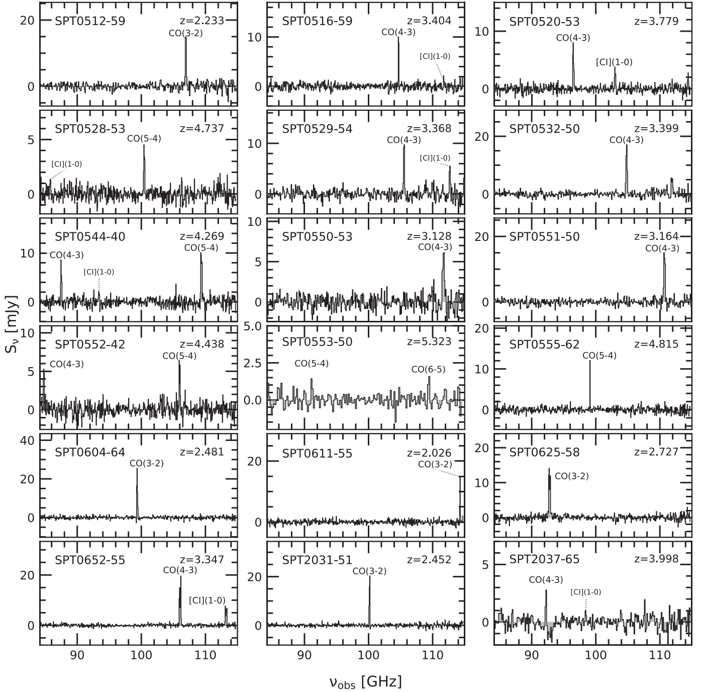
Figure B3. The 3 mm ALMA spectra (spanning 84.2–114.9 GHz) of all SPT DSFGs. Marginal detections ( >3\sigma ) are designated by the smaller font and dashed line.
