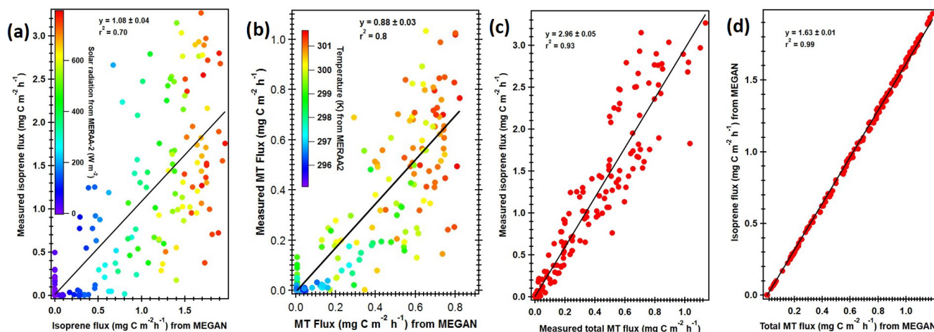
Figure 5. Scatterplots for measured and MEGAN2.1 estimated isoprene and total monoterpene fluxes and their correlations.
