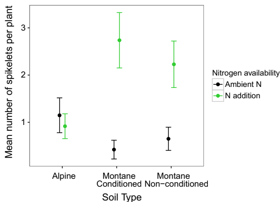
Fig. 3 Means and standard errors of B. tectorum spikelet production per plant (including plants with zero spikelets). We pooled freezing temperature treatments because we did not detect an effect of freezing temperature on spikelet production. The N addition treatment pots received the equivalent of 20 \text{ kg N ha}^{-1} \text{ year}^{-1}
