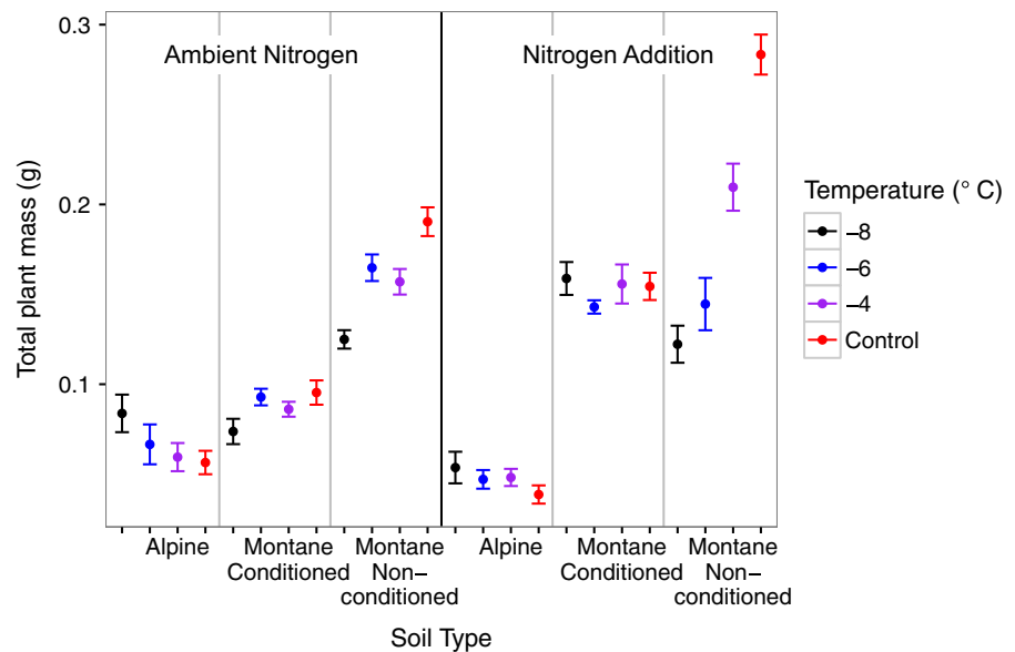
Fig. 2 Means and standard errors of B. tectorum total dry plant mass at the end of the freeze recovery experiment. The N addition treatment pots received the equivalent of 20 \text{ kg N ha}^{-1} \text{ year}^{-1} . The control freezing temperature was 5^\circ\text{C} which was the nighttime temperature experienced by all plants during the growing and recover phases of the experiment
