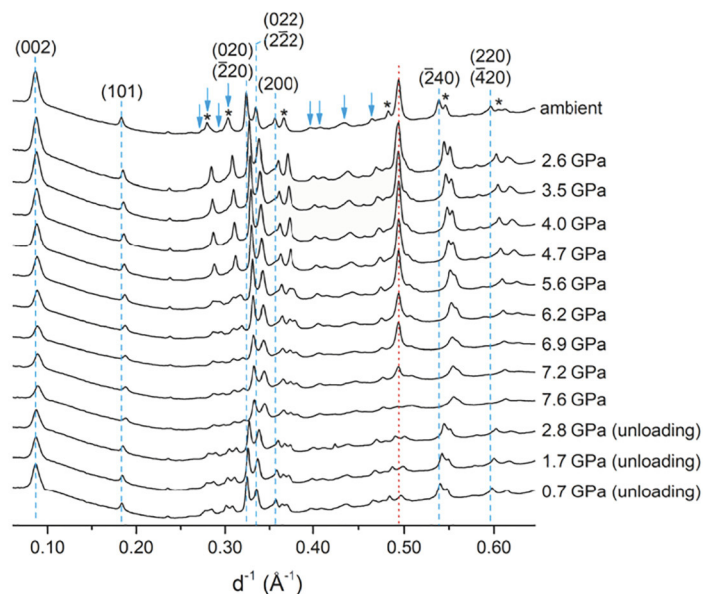
Fig. 4. X-ray diffractogram of A) single-chain Al-free 11 \text{\AA} tobermorite, B) double-chain Al-free tobermorite, C) double-chain tobermorite Al/(Al + Si) = 1/12, D) double-chain tobermorite Al/(Al + Si) = 1/6 as a function of applied hydrostatic pressure. The tobermorite peaks, which were not used for refinement, are indicated with blue arrows. The impurities are labeled with asterisk (vaterite), cross (calcite), and pound sign (aragonite). The red dot line indicates the diffraction from the gasket. (For interpretation of the references to color in this figure legend, the reader is referred to the web version of this article.)
