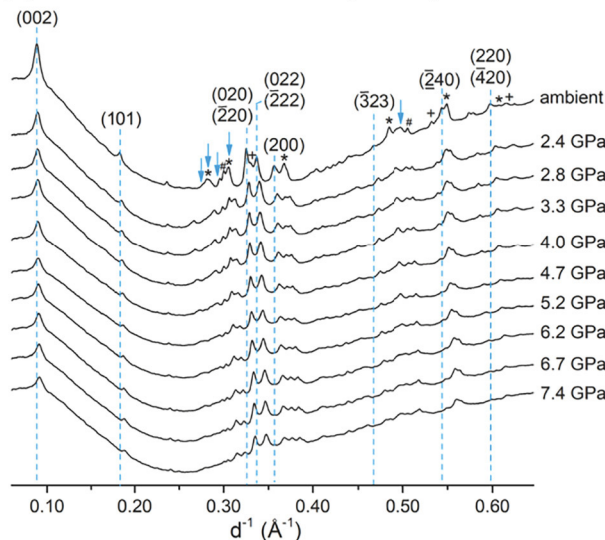
Fig. 4. X-ray diffractogram of A) single-chain Al-free 11 \text{\AA} tobermorite, B) double-chain Al-free tobermorite, C) double-chain tobermorite Al/(Al + Si) = 1/12, D) double-chain tobermorite Al/(Al + Si) = 1/6 as a function of applied hydrostatic pressure. The tobermorite peaks, which were not used for refinement, are indicated with blue arrows. The impurities are labeled with asterisk (vaterite), cross (calcite), and pound sign (aragonite). The red dot line indicates the diffraction from the gasket. (For interpretation of the references to color in this figure legend, the reader is referred to the web version of this article.)
