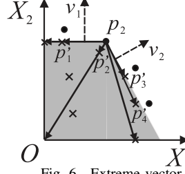
Fig. 6. Extreme vector
