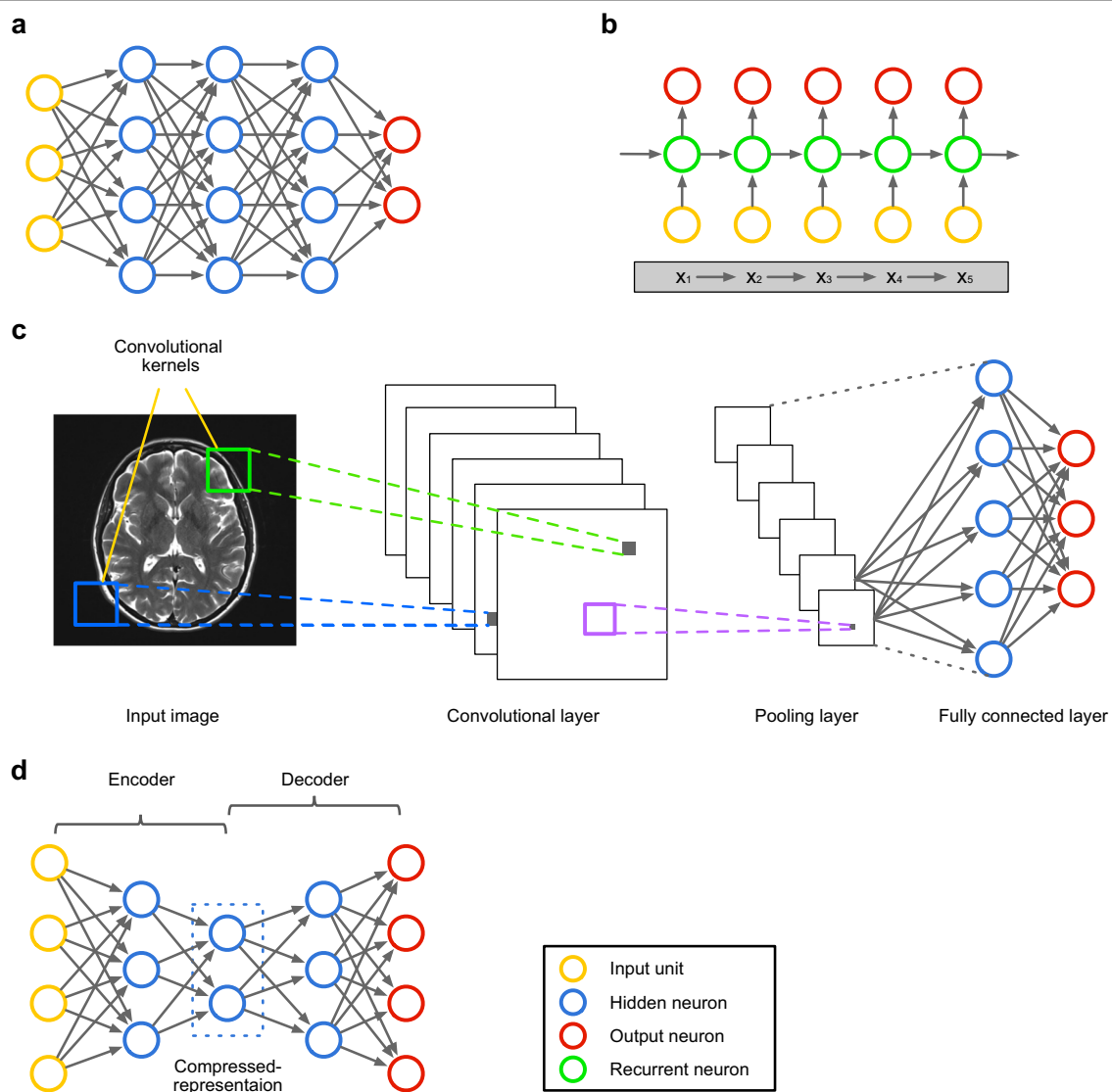
Fig. 1 Examples of deep neural networks. a Deep feedforward neural network (DFNN). It is the basic design of DL models. Commonly, a DFNN contains multiple hidden layers. b A recurrent neural network (RNN) is presented to process sequence data. To encode history information, each recurrent neuron receives the input element and the state vector of the predecessor neuron, and yields a hidden state fed to the successor neuron. For example, not only the individual information but also the dependence of the elements of the sequence x_1 \rightarrow x_2 \rightarrow x_3 \rightarrow x_4 \rightarrow x_5 is encoded by the RNN architecture. c Convolutional neural network (CNN). Between input layer (e.g., input neuroimage) and output layer, a CNN commonly contains three types of layers: the convolutional layer that is to generate feature maps by sliding convolutional kernels in the previous layer; the pooling layer is used to reduce dimensionality of previous convolutional layer; and the fully connected layer is to make prediction. For the illustrative purpose, this example only has one layer of each type; yet, a real-world CNN would have multiple convolutional and pooling layers (usually in an interpolated manner) and one fully connected layer. d Autoencoder consists of two components: the encoder, which learns to compress the input data into a latent representation layer by layer, whereas the decoder, inverse to the encoder, learns to reconstruct the data at the output layer. The learned compressed representations can be fed to the downstream predictive model.
