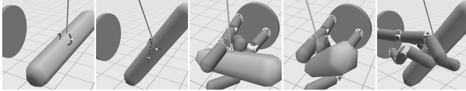
Fig. 14: (a) displays the floating contacts for the acceptable sphere rotation, capsule rotation and translation motion example, while (b) displays a different version of this motion obtained via a different set of initial contact points. The contacts in (a) do not cause the attached fingers to self-collide, while it is impossible to construct fingers to follow the trajectories in (b) without self collision. (c) displays the non-colliding example, while (d) displays the colliding example after the "whole hand" optimization stage. The "whole hand" planner was unable to find an alternate solution in (d) with the mechanism given to it that did not involve finger collision, and as a result the solution it found involves the fingers passing through one another.
