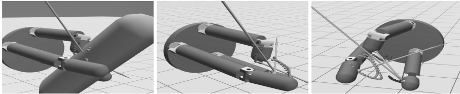
Fig. 10: As figures (a) and (b) show (on our rotate and bow out single objective motion), with L_{frictionConeHand} removed from our whole hand optimization, even slight collision between the fingertip and object can cause very unrealistic contact forces with respect to the fingertip's frame. Figure (c) shows the same optimization with L_{frictionConeHand} included, indicating that it prevents this type of inconsistency from occurring.
