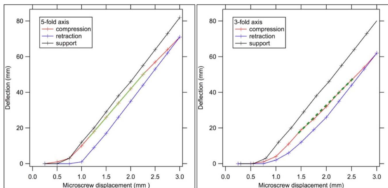
Fig 7. Indentation of the magnetic cage model with a small force, at 2 different cage orientations: 5-fold (left) and 3-fold (right). The black curve is obtained by compressing the substrate directly. The green line is a linear fit to the compression curve for the 5-fold orientation, and the dashed green line is a linear fit for the 3-fold orientation. The slope of the linear fit gives the sample stiffness. The 5-fold orientation corresponds to a steeper slope, and, thus, the highest stiffness.
