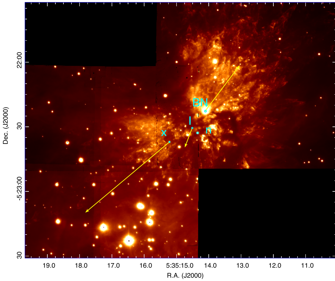
Figure 1. A 2.12\ \mu\text{m} narrowband \text{H}_2 image from Bally et al. (2015) showing Src x, Src I, BN, and Src n. The yellow arrows show the proper motions of the three ejected stars with lengths corresponding to the motions over the next 2000 yr. The vectors shown are based on the motions measured by Rodríguez et al. (2017) for the BN object and Src I, and by Luhman et al. (2017) for Src x. The Trapezium cluster of massive stars in the center of the Orion Nebula are located near the bottom of the image.
