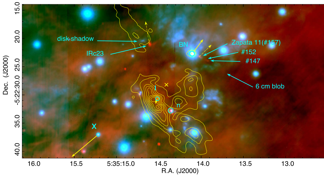
Figure 5. A color composite image showing a portion of the 6 GHz radio continuum from Forbrich et al. (2016) in red, superimposed on the 1.64\ \mu\text{m} [Fe II] image from Bally et al. (2015) in cyan. Yellow contours show the 1.3 mm dust continuum emission from OMC1 at 1'' resolution (Bally et al. 2017) with contour levels at 50, 156, 261, 367, 472, 578, 683, 689, 789, and 894 mJy/beam (the beam has an FWHM of about 1'' ). The solid yellow arrows mark the proper motions of the ejected stars with lengths corresponding to the motion over the next 200 yr. Dashed arrows show the proper motions of E2 (“IRc 23”) and SW1 (“Zapata 11”) taken from Dzib et al. (2017). The “X” marks the center of the explosion as determined by Bally et al. (2011, 2015, 2017). The radio emission feature labeled “IRc 23” lies at the western edge of the cometary clump of dust pointing roughly to the explosion center. A compact bipolar reflection nebula with an axis at PA \sim 100^\circ shows the location of a “disk shadow,” presumably illuminated by an obscured central star located in the head of the cometary dust feature. The numbered 6 GHz sources (#152 and #147) southwest of BN were tabulated by Forbrich et al. (2016). The “6 cm blob” is an extended enhancement of radio continuum emission along the axis defined by Zapata 11, #152, and #147.
