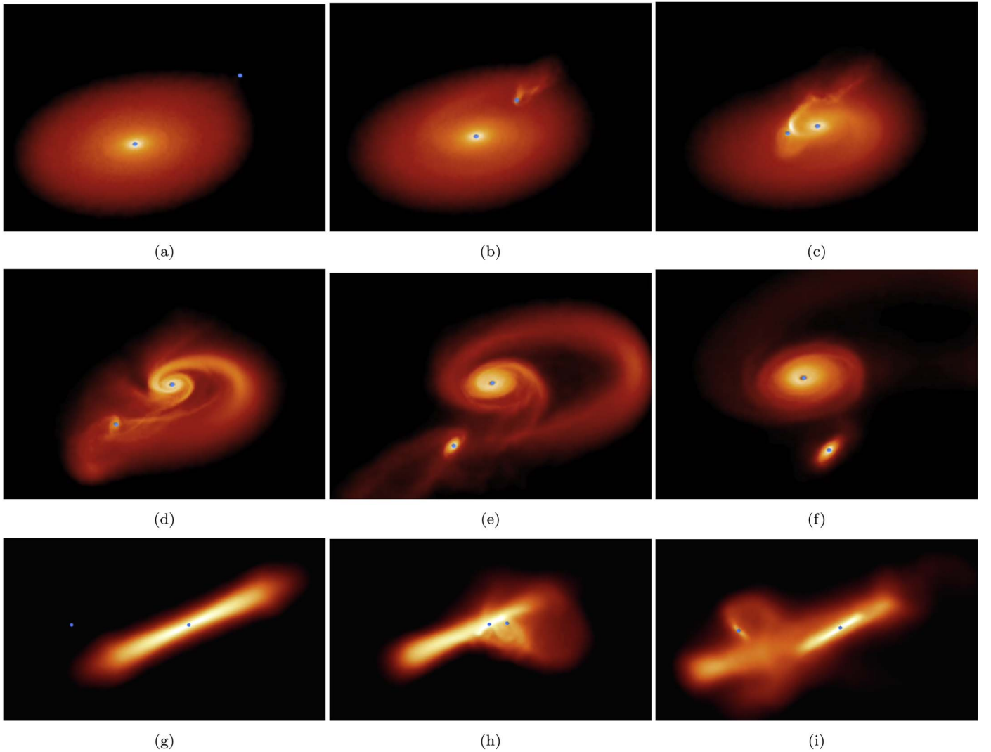
Figure 7. (a) through (f): snapshots of an SPH simulation showing the evolution of the first encounter of a 5 M_{\odot} intruder star with no disk in an initially hyperbolic orbit inclined by 30^{\circ} with respect to the disk plane around a 15 M_{\odot} star. Orbital energy dissipation traps the intruder into an inclined, elliptical orbit around the primary. The total mass of the disk is 1.5 M_{\odot} . The gravitational radius of the 5 M_{\odot} intruder star is r_G \approx 0.17r , where r is the distance from the 15 M_{\odot} star. Frames taken from simulations used in Cunningham et al. (2009) and Moeckel & Bally (2006, 2007). (g) through (i): frames (a), (c), and (e) above seen from a vantage point located to the right in frames (a) through (f) and lying in the initial disk plane of the massive star.
