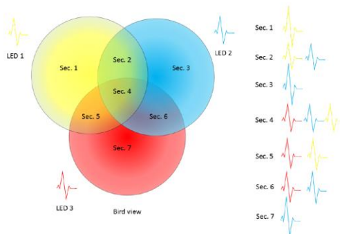
Fig. 5. A simple proximity method for VLP tracking [15].
