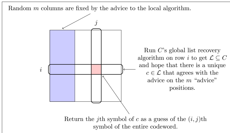
FIG. 1. The local algorithm A_{(c_1, \dots, c_m)} , for C \otimes C on input (i, j) \in [n] \times [n] . Here, c_1, \dots, c_m are “advice”: c_i \in \mathcal{L}_i is one of L possible codewords for the i th randomly selected column. The set of selected columns is random, but we have shown them as the first m columns for simplicity.
