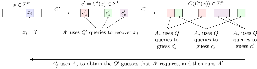
FIG. 2. The local algorithm A'_j used in the proof of Lemma 3.1.
