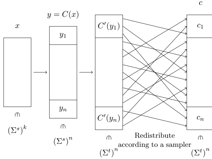
FIG. 3. The construction of [GKO + 18]. A message x \in (\Sigma^s)^k is encoded into a codeword y = C(x) \in (\Sigma^s)^n . Then each symbol is encoded with an inner code C' : \Sigma^s \rightarrow \Sigma^t . Finally, the symbols from \Sigma are redistributed according to a sampler. More precisely, if (u, v) is an edge in the sampler, so that v is the i th neighbor of u and u is the j th neighbor of v , then the j th symbol in c_v is defined to be the i th symbol of y_u .
