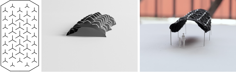
Figure 1: Our printing-on-fabric meta-material encodes surface curvature within a regular star pattern (left). Our predictive simulation allows the virtual design of architectural models (middle), with a close match to physical realization (right).
