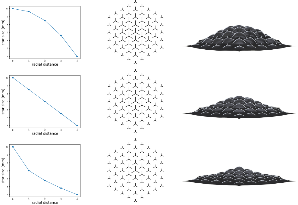
Figure 9: Effect of different arm-length gradient profiles on the equilibrium shape of a hexagonal star pattern. Each row corresponds to a different function \ell(x,y) : on the left, a plot of \ell as a function of distance to the hexagon center; in the middle, a diagram of the corresponding star pattern design; and on the right, the simulated equilibrium shape.
