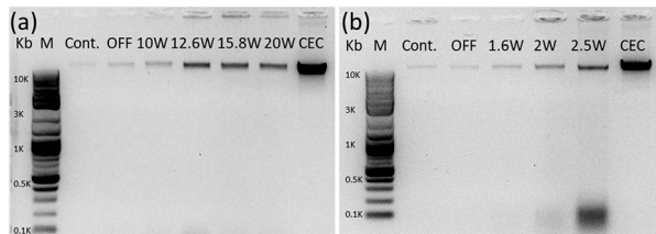
Fig. 5 Agarose gel electrophoresis analysis of nucleic acids extracted at indicated TSAW power level. (a) Traveling surface acoustic waves at frequency of 13 MHz. (b) Traveling surface acoustic waves at frequency of 160 MHz. The no-lysis control ("Cont.") is generated from bacteria kept on ice. The complete extraction control ("CEC") is prepared using the Bacterial Genomic DNA kit. "M" is 100 bp DNA ladder; "kb" is kilobases.
