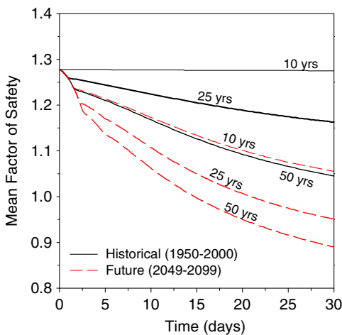
Fig. 8. Mean factor of safety for slope stability versus time using the historical and future 10-, 25-, and 50-year flood simulations.
