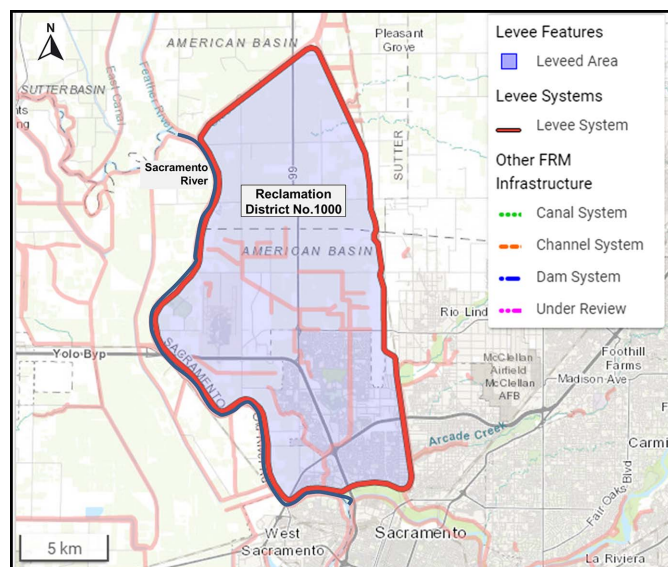
Fig. 1. Leveled area in Reclamation District No. 1000, Sacramento, California. (Reprinted from NLD 2020.)
