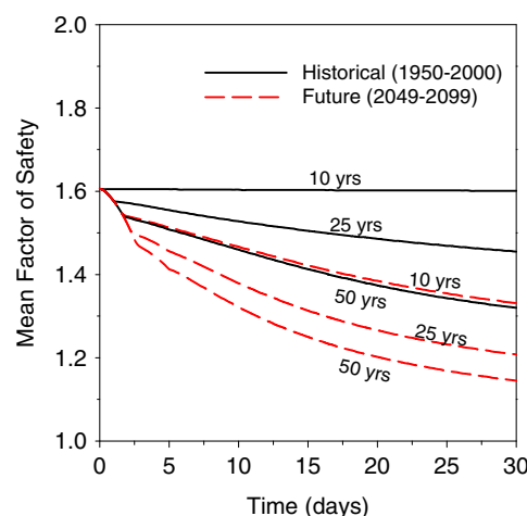
Fig. 6. Mean factor of safety for uplift at the toe versus time using the historical and future 10-, 25-, and 50-year flood simulations.
