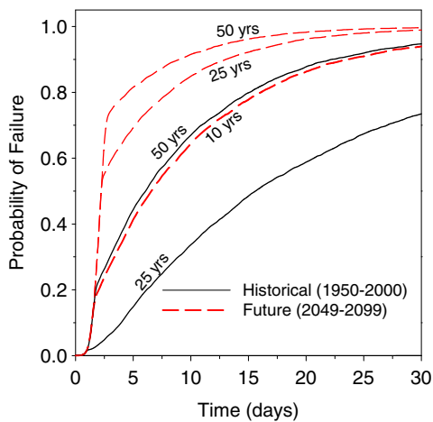
Fig. 7. Probability of failure for uplift at the toe versus time using the historical and future 10-, 25-, and 50-year flood simulations.
