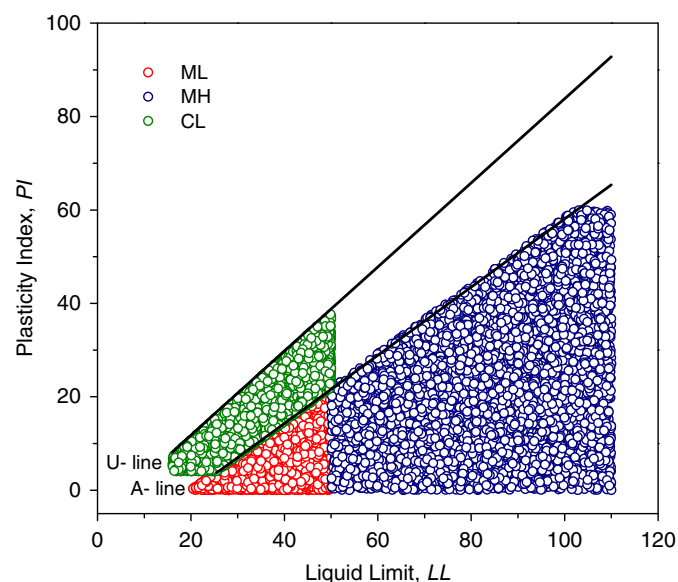
Fig. 3. Correlated random samples of LL and PI used in simulation. (Data from Schultz et al. 2018.)
