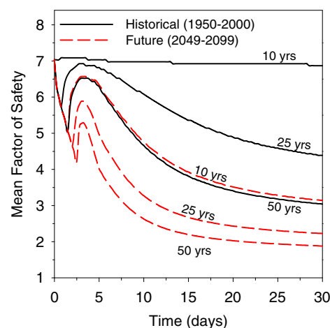
Fig. 4. Mean factor of safety for underseepage at the toe versus time using the historical and future 10-, 25-, and 50-year flood simulations.
