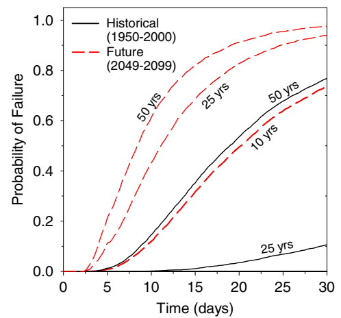
Fig. 9. Probability of failure for slope stability versus time using the historical and future 10-, 25-, and 50-year flood simulations.
