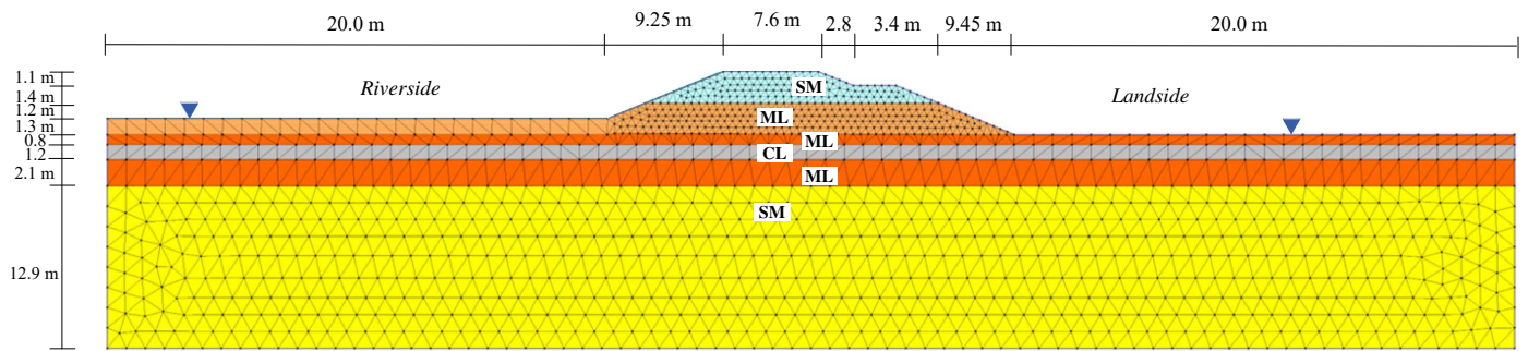
Fig. 2. Geometry of Elkhorn Levee used in numerical modeling.
