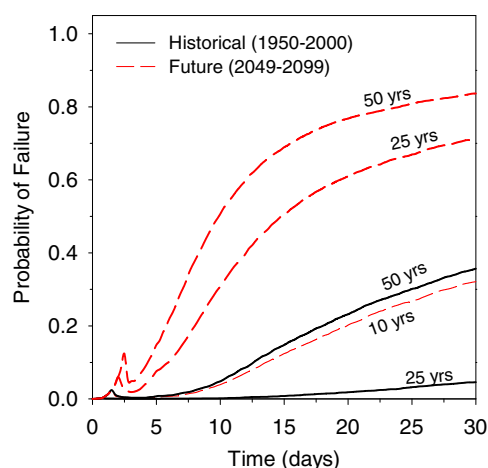
Fig. 5. Probability of failure for underseepage at the toe versus time using the historical and future 10-, 25-, and 50-year flood simulations.
