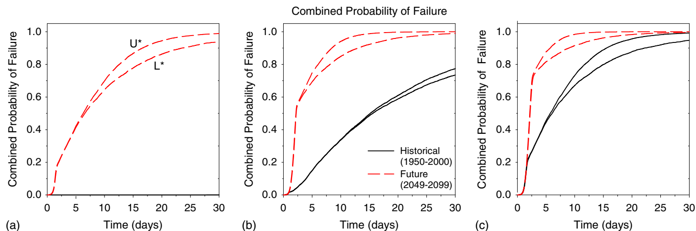
Fig. 10. Upper and lower bounds for combined probability of failure versus time using the historical and future flood scenarios for different recurrence intervals: (a) 10 years; (b) 25 years; and (c) 50 years.
