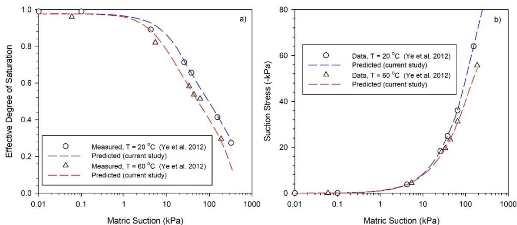
Fig. 5. Experimental and predicted data of effective degree of saturation and suction stress for GMZ01 bentonite at temperatures 20°C and 60°C
