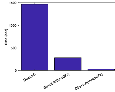
Figure 7: Execution time of DIRECT-E, DIRECT-A ( \tau=2067 ), and DIRECT-A ( \tau=20672 ) in p2p-3
