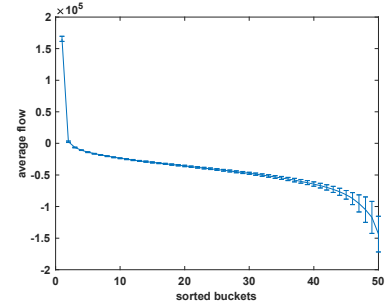
Figure 8: Absolute Error of the DIRECT-A ( \tau = 20672 ) in p2p-3
