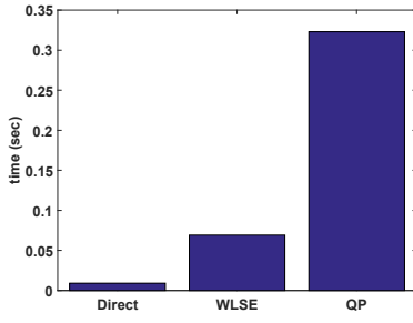
Figure 6: DIRECT v.s. baselines in N_1 : n = 281 and m = 827
