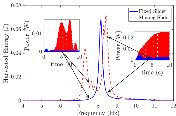
FIG. 4. Total energy harvested over 10 s with and without a sliding mass for a range of frequencies s_0 = 0.5L .
