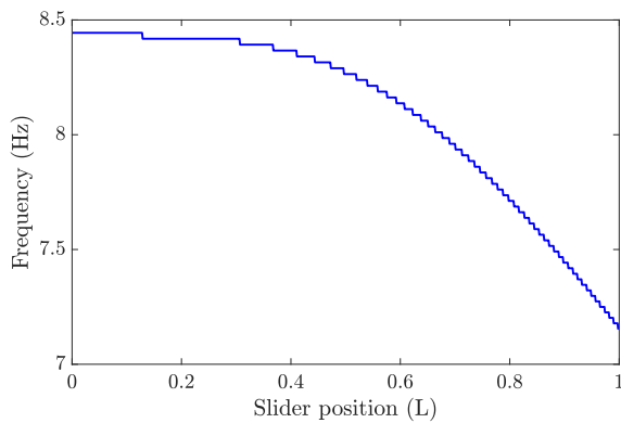
FIG. 2. Fundamental natural frequency of the system varies between 7.2 Hz and 8.4 Hz with changing slider position.
