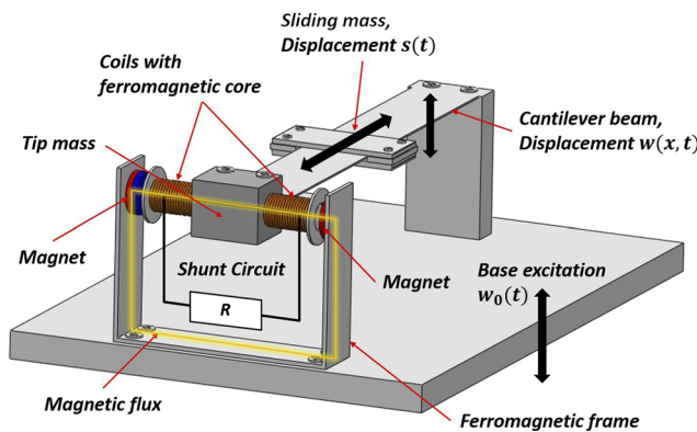
FIG. 1. Key components of the self-tuning vibration energy harvesting system.
