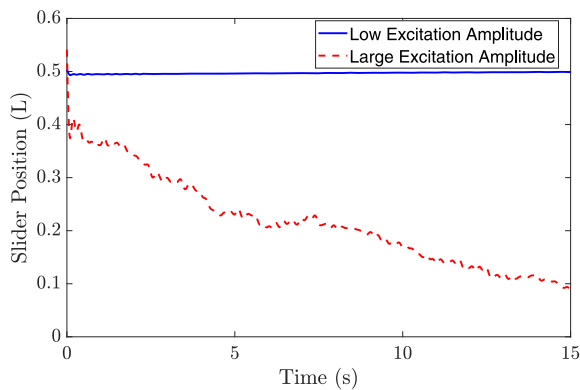
FIG. 7. Measured position of the slider at a high excitation frequency for low and high excitation amplitudes (10.25 Hz).
