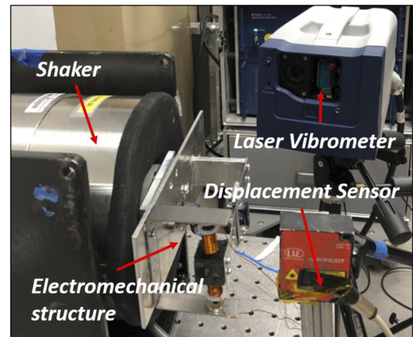
FIG. 5. Key components of the experimental setup.
