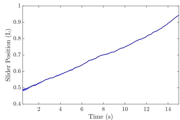
FIG. 6. Measured position of the slider at a low excitation frequency (8.25 Hz).
