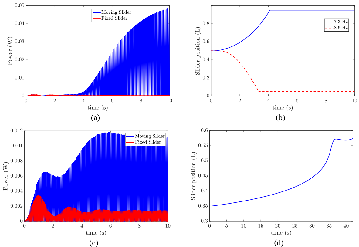
FIG. 3. Simulation results at different excitation frequencies: (a) Harvested power at 7.3 Hz; (b) slider position at 7.3 Hz and 8.6 Hz; (c) harvested power at 8.6 Hz; and (d) slider position at frequencies close to the second vibration mode at 72.2 Hz.
