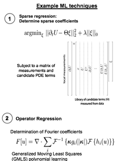
Fig. 6 ML techniques applicable to model derivation (1) sparse regression [Image courtesy of E.P. Alves and F. Fiuza, SLAC], and (2) operator regression [56]
